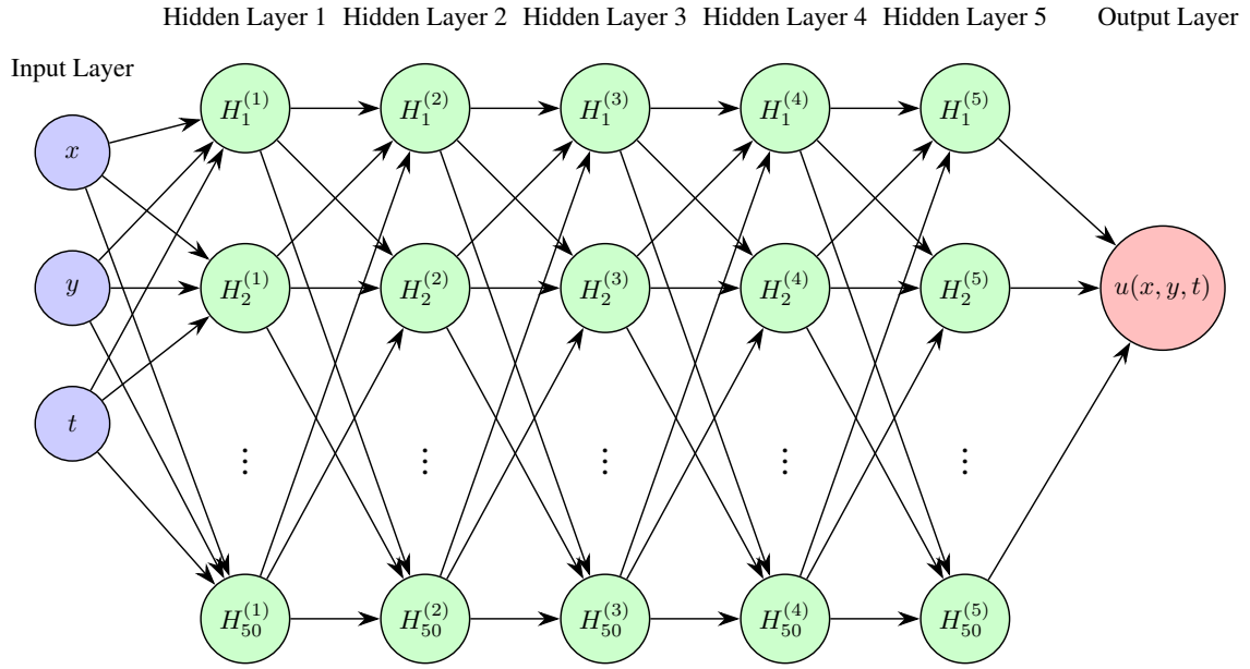
Figure 2: The Physics informed neural Network (PINN). This Figure 2 shows the architecture of the Physics informed neural Network (PINN) to calculate the heat conduction problem (30, 31, 32). This PINN contains three input nodes, five hidden layers, each of them containing 50 nodes. The output layer has one output node containing the result u(x, y, t) . A hyperbolic tangent function as activation is used.
