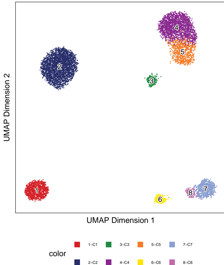
UMAP of IterativeLSI colored by colData : Clusters
