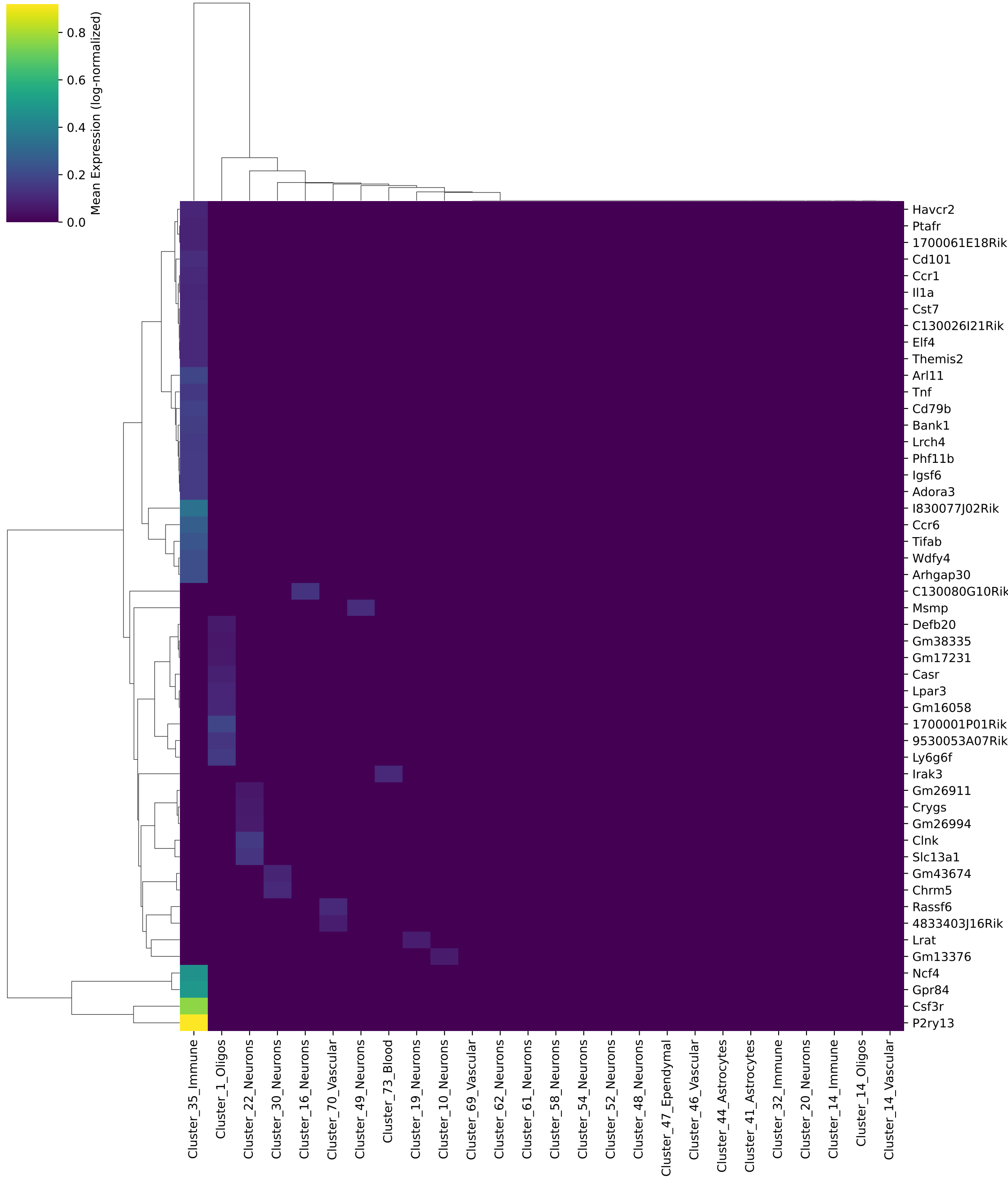
Top 50 DEGs: Expression Across Cell Types
