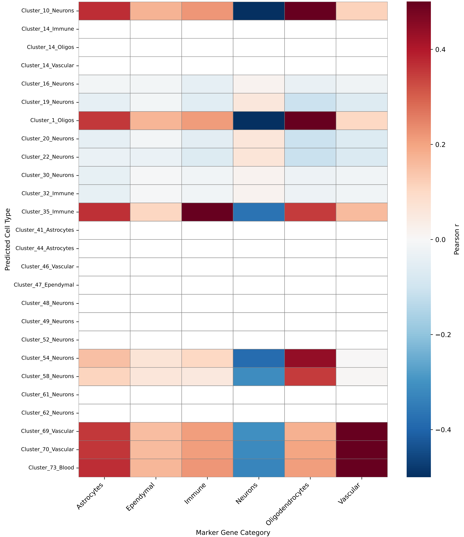
Marker Gene Validation: Correlation Heatmap (Marker Expression vs Predicted Proportions)
