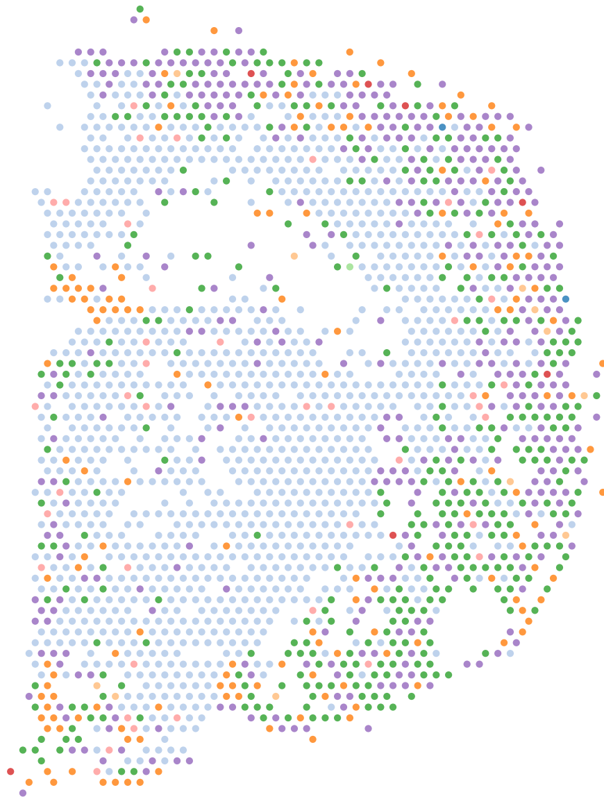
Dominant Cell Type per Spot
