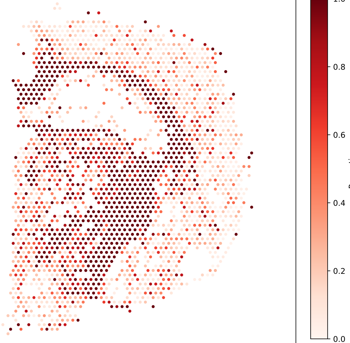
Confidence (Proportion of Dominant Type)
