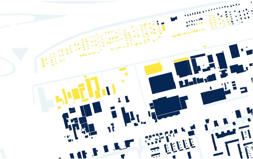
RTM local transition structure
