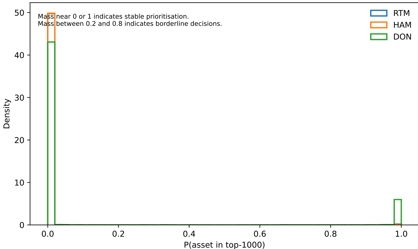
Posterior top-k membership probability, k=1000
