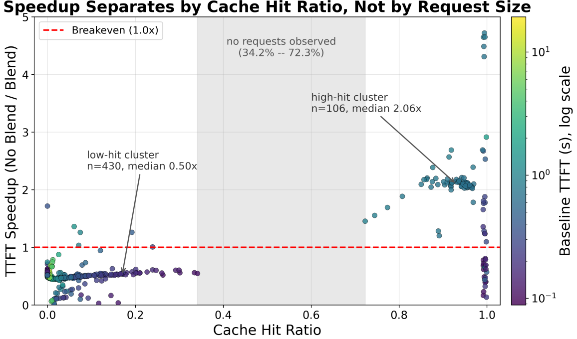
Figure 4.1: Per-request TTFT speedup against cache hit ratio, coloured by baseline TTFT. The two populations are separated by a band of hit ratios in which the trace contains no observations. Four requests above 5\times are outside the plotted range; cluster statistics are computed over all requests.
