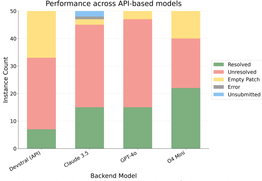
Figure 4.9: Resolve rate distributions for SWE-bench Verified-mini evaluation runs across different models.
