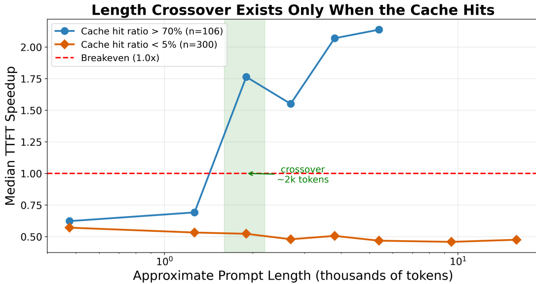
Figure 4.7: Median TTFT speedup vs. prompt length, split by cache hit ratio. A length crossover near 2,000 tokens exists for requests that hit the cache. For requests that miss, the penalty is flat at \sim 0.5\times across the entire length range, so no length threshold recovers them. The hit-ratio series ends near 6,000 tokens because the trace contains almost no well-cached prompts beyond that length. Prompt length is estimated from baseline TTFT, which is a near-linear proxy (Pearson r = 0.99 on the subset with recorded token counts).
