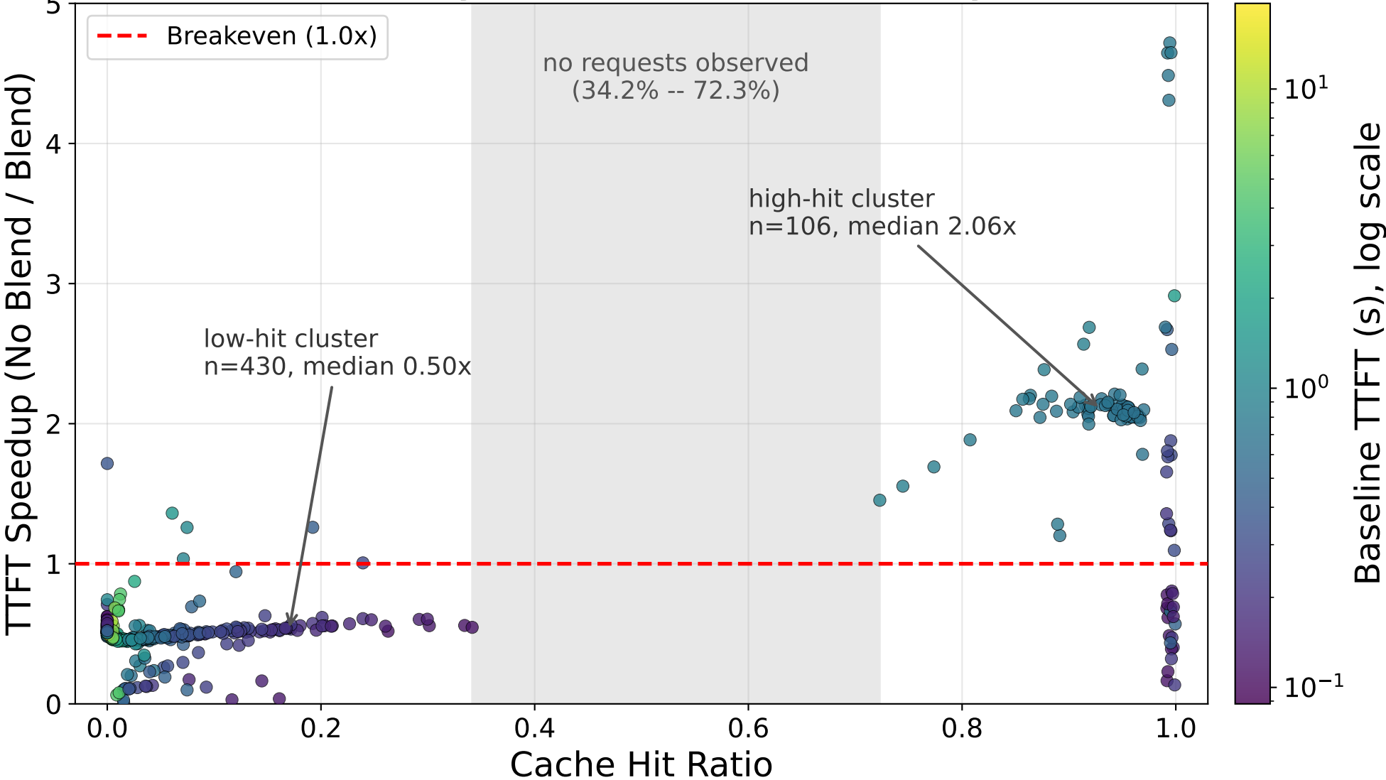
Speedup Separates by Cache Hit Ratio, Not by Request Size
