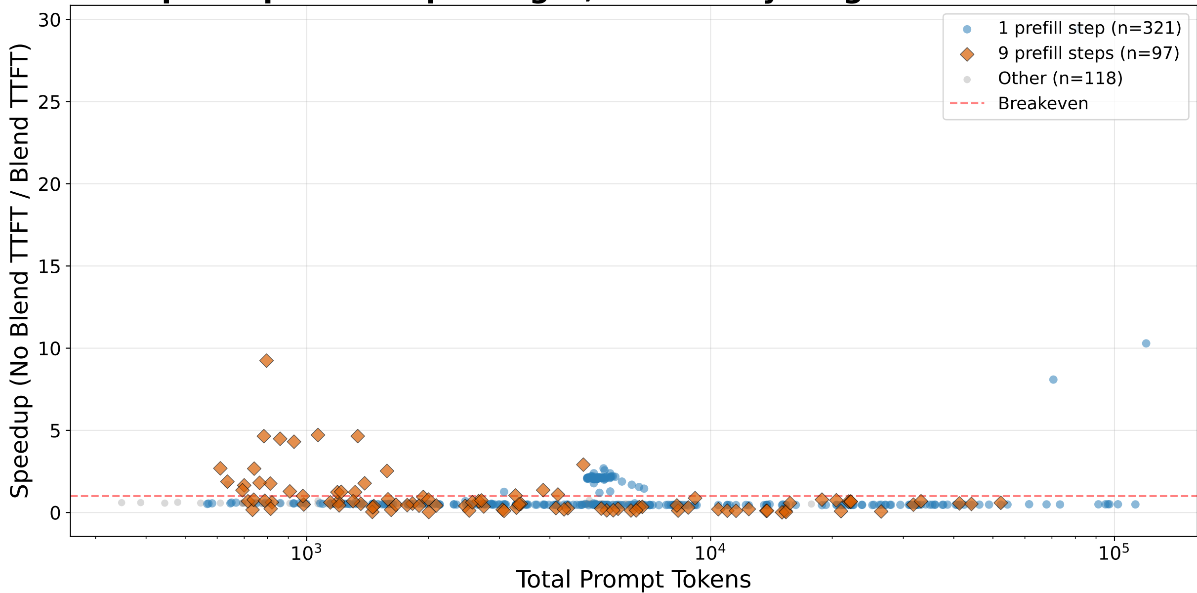
Speedup vs Prompt Length, Colored by Fragmentation Class
