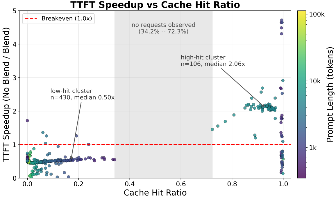
Figure 4.2: Per-request TTFT speedup against cache hit ratio, coloured by prompt length in tokens. Speedup separates by cache hit ratio, not by request size: both clusters span the full length range, and the two populations are divided by a band of hit ratios in which the served run contains no observations. Four requests above 5\times are outside the plotted range; cluster statistics are computed over all requests.
