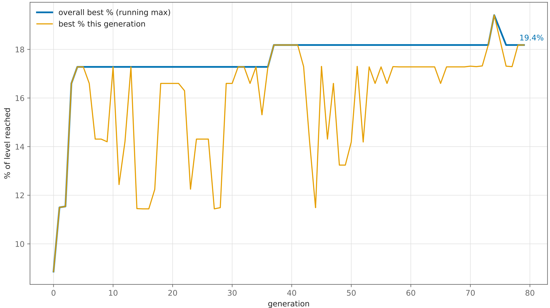
Learning curve — how far the best network gets over generations
