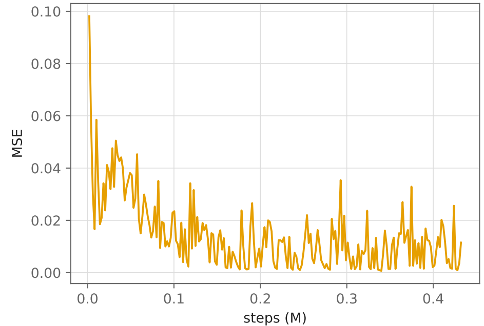
Value loss — can the critic predict returns?
