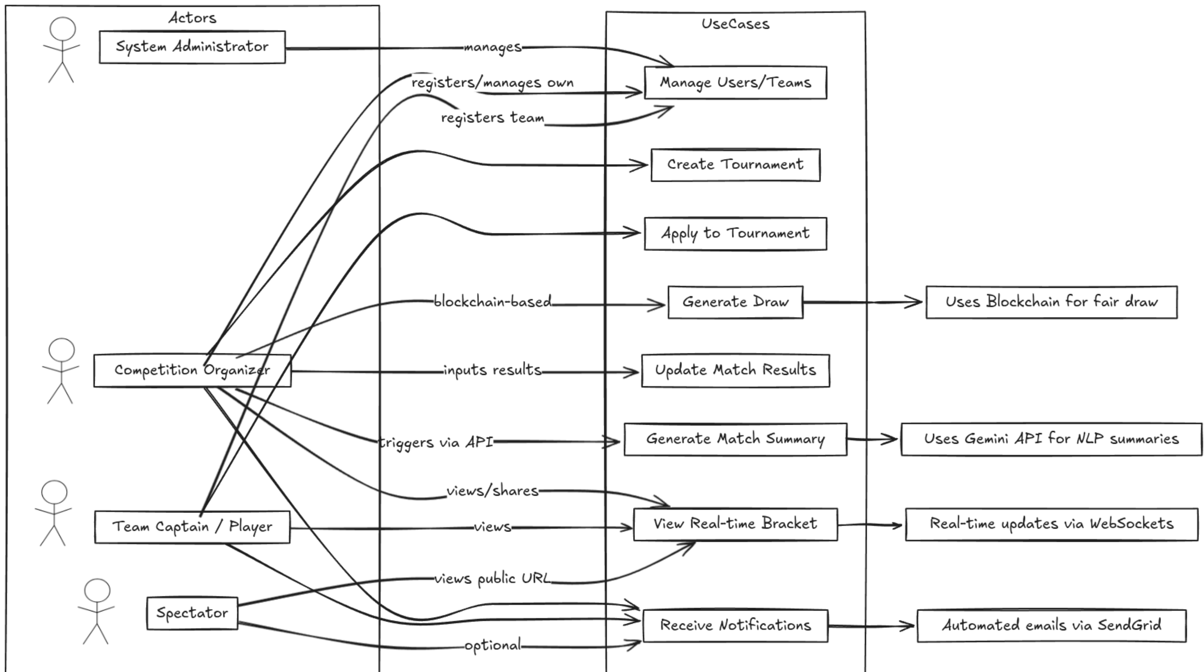
Use Case Diagram for Project Aegis MVP
