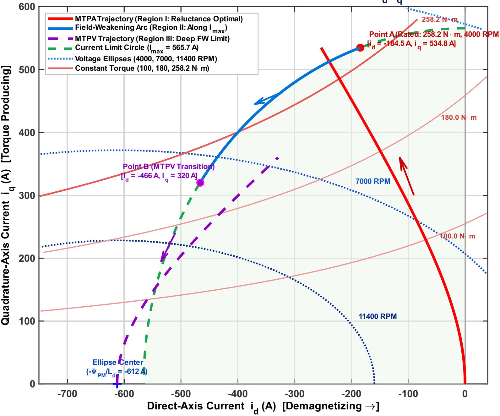
MTPA & MTPV Vector Control Operating Envelope in ( i_d , i_q ) Plane
