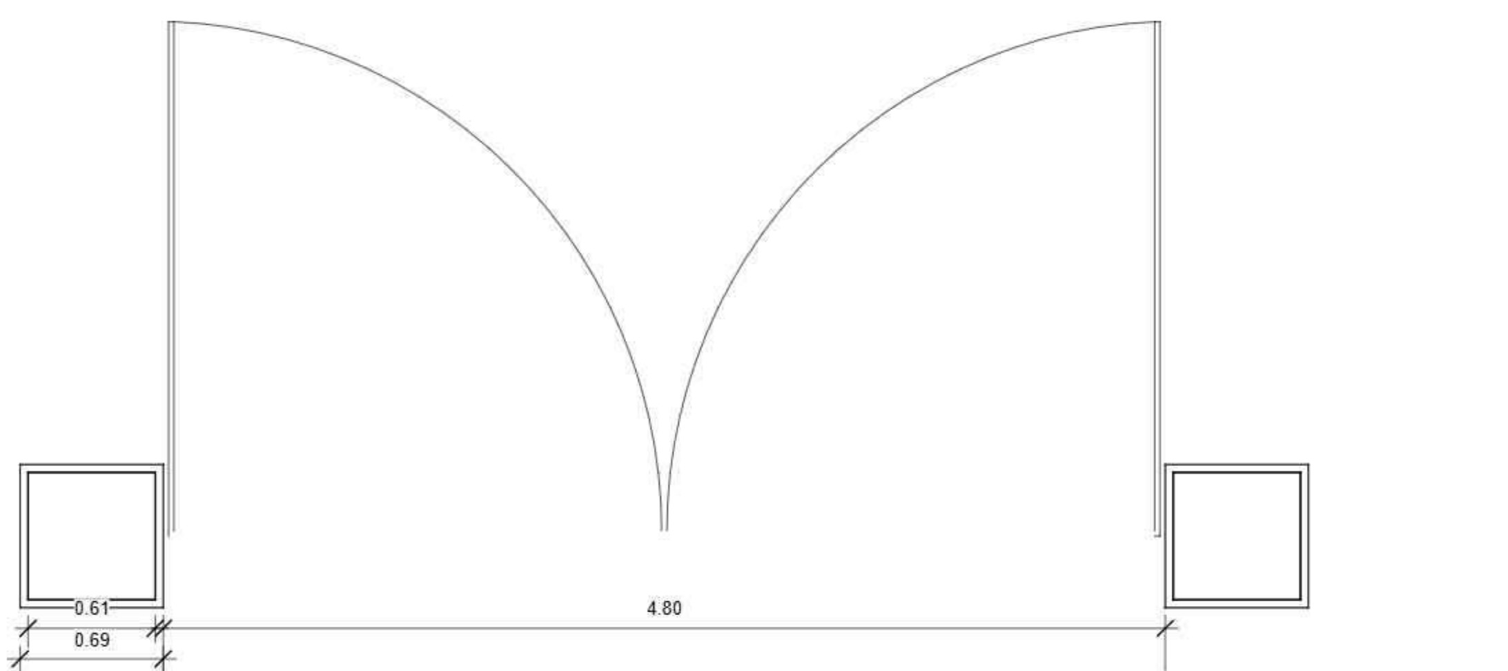
Entrance fence 1 : 25
