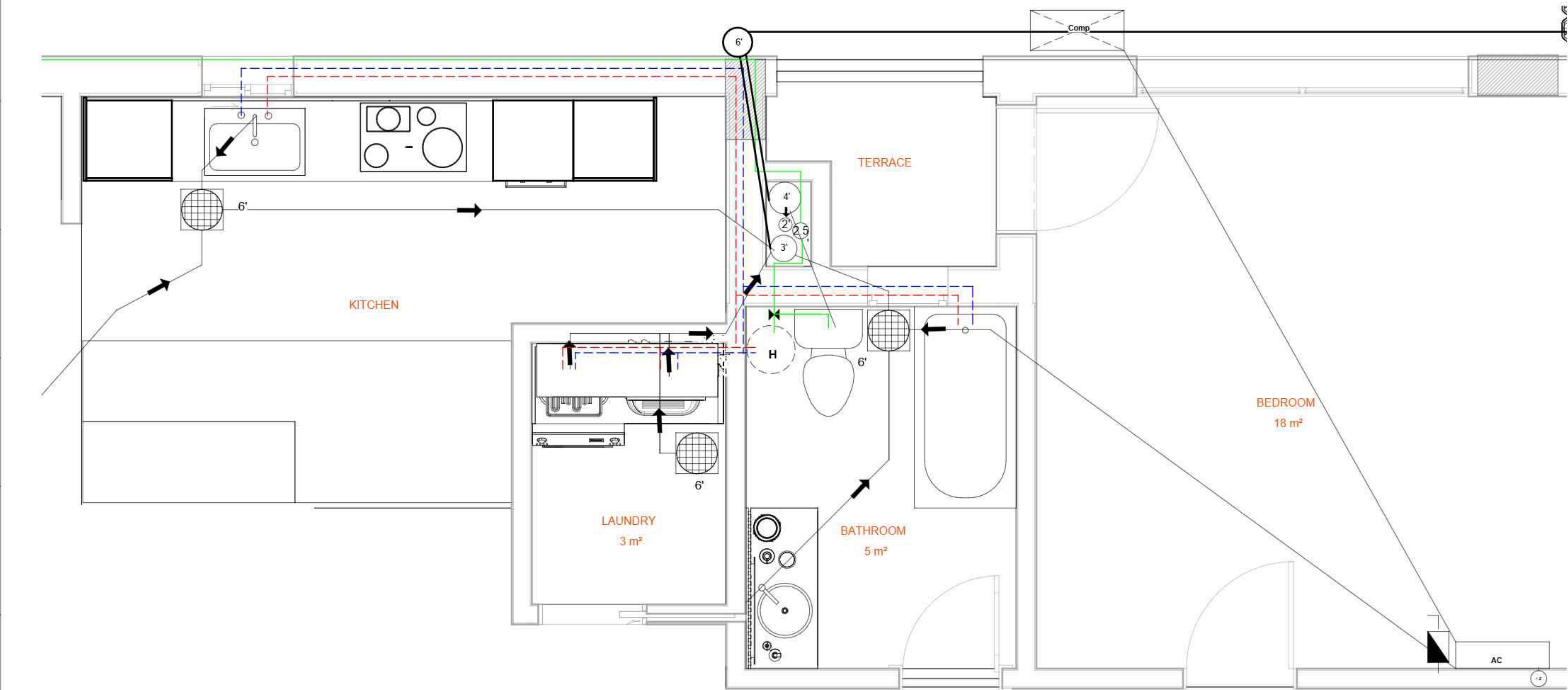
Ground Floor Plan (Plumbing) - Callout 1 1 : 20
