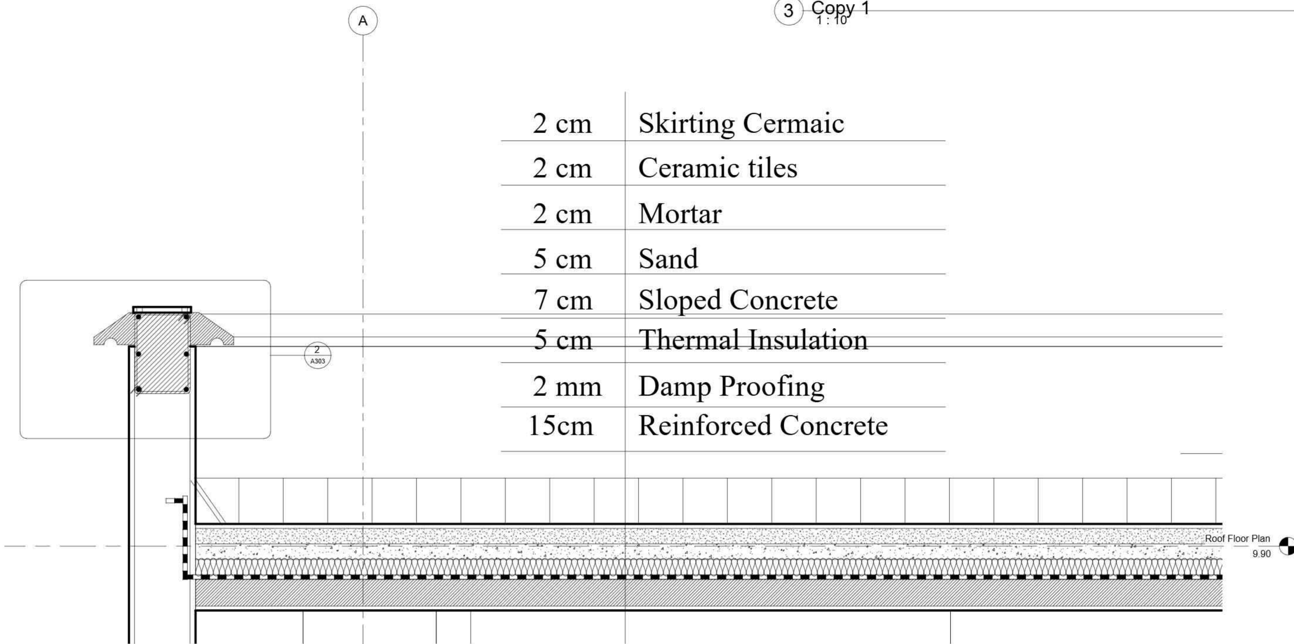
3 Bathroom Flooring Layers Copy 1 1 : 10
