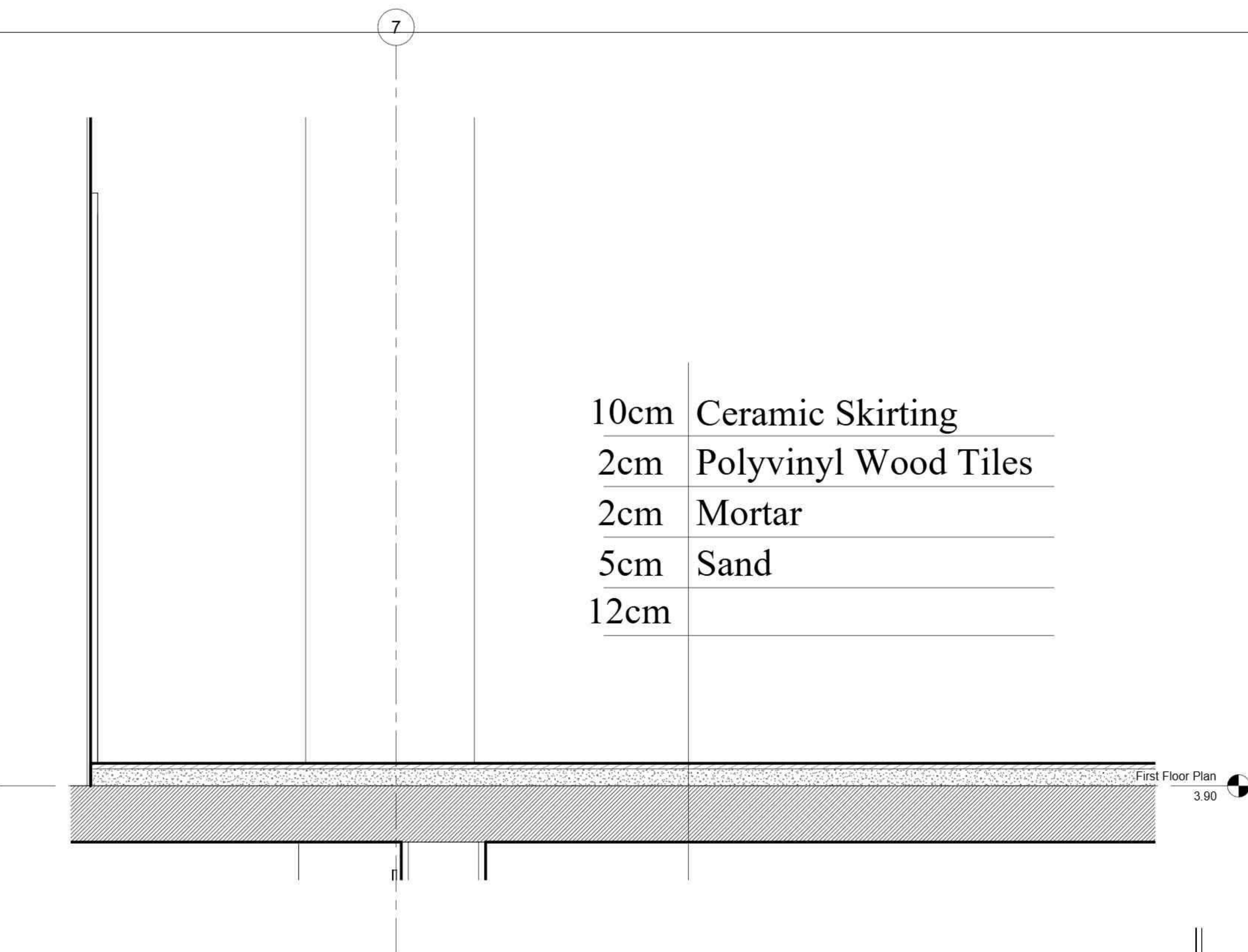
1 Typical Floor Layers 1 : 10
