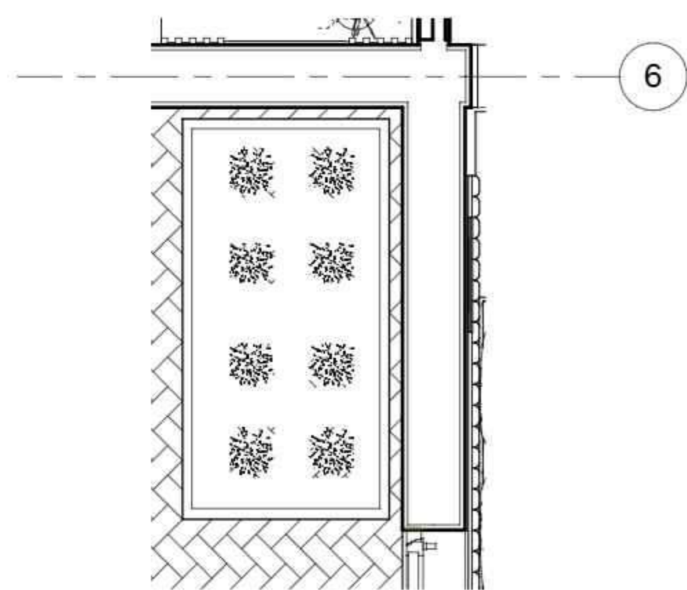
4 Flower Box at Entrance 1 : 25
