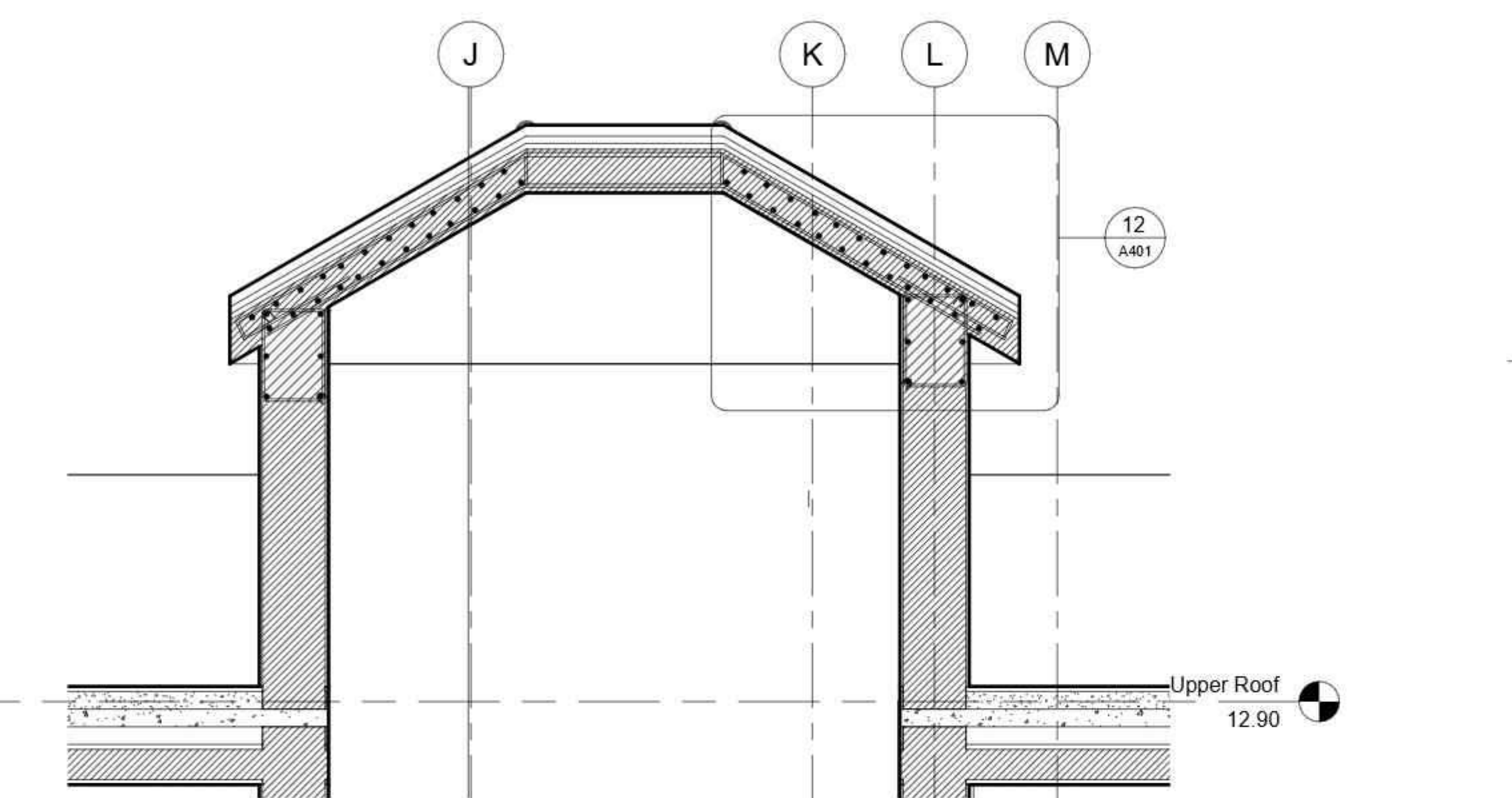
Pitched Roof Detail 1 : 20
