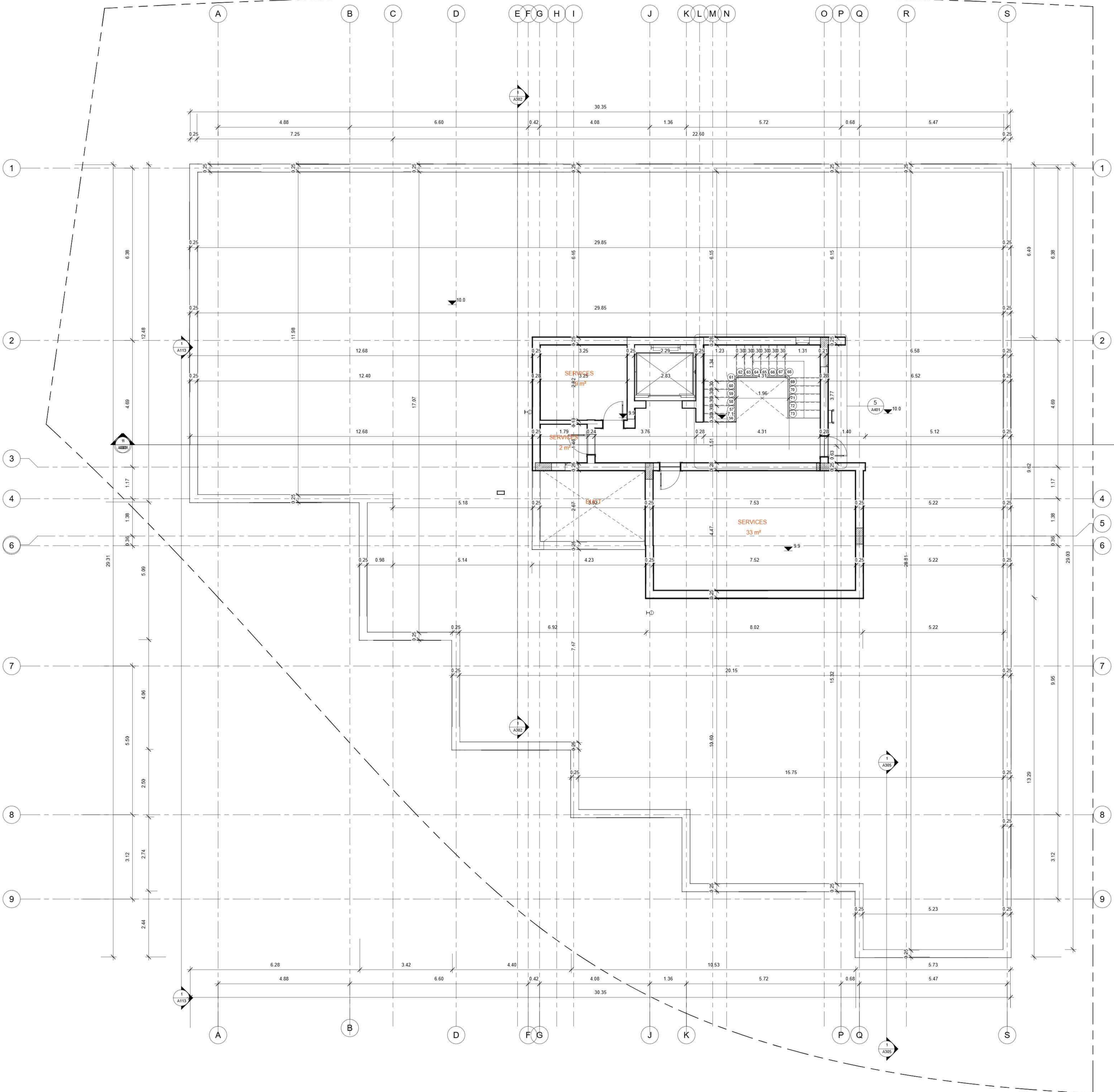
1 Roof Floor Plan 1 : 50
