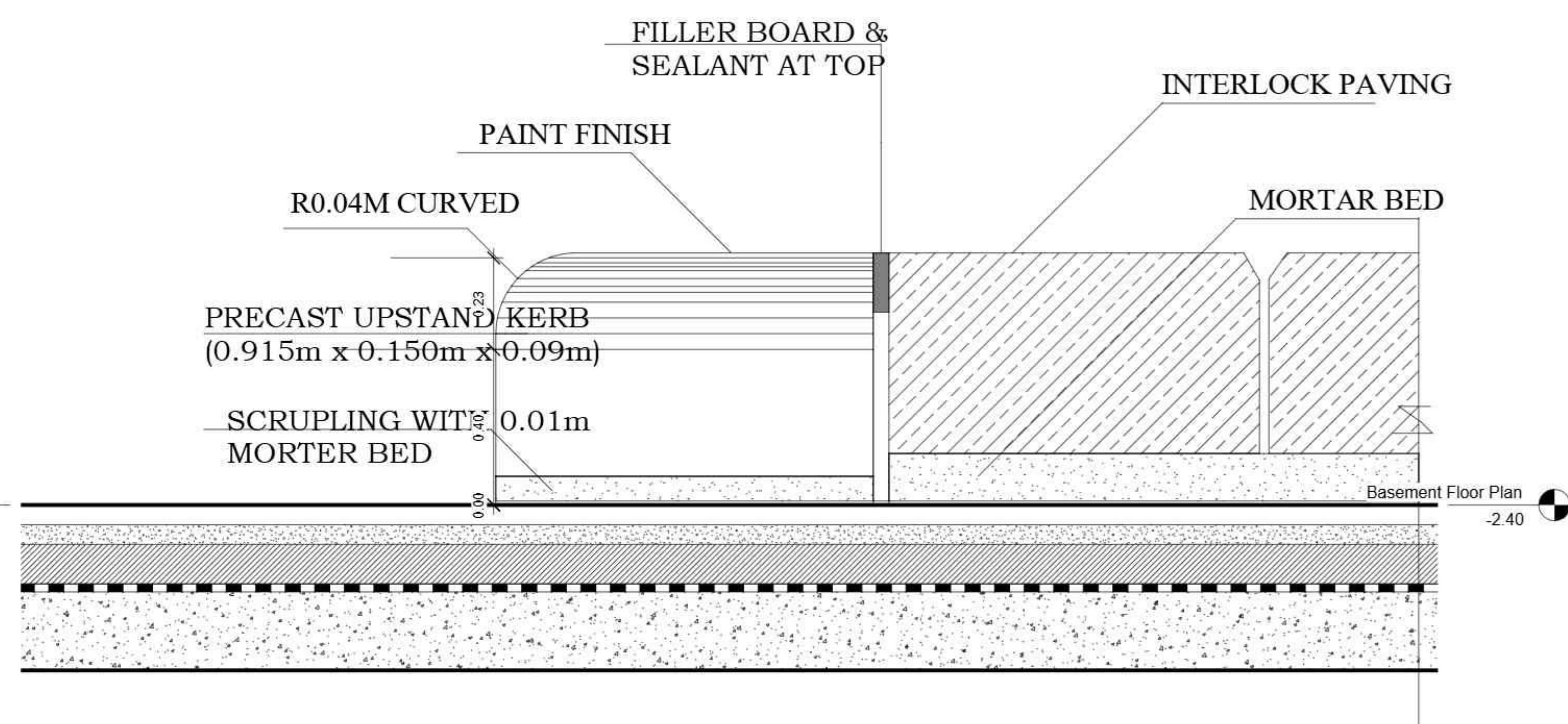
4 Kerb Detail 1 : 10
