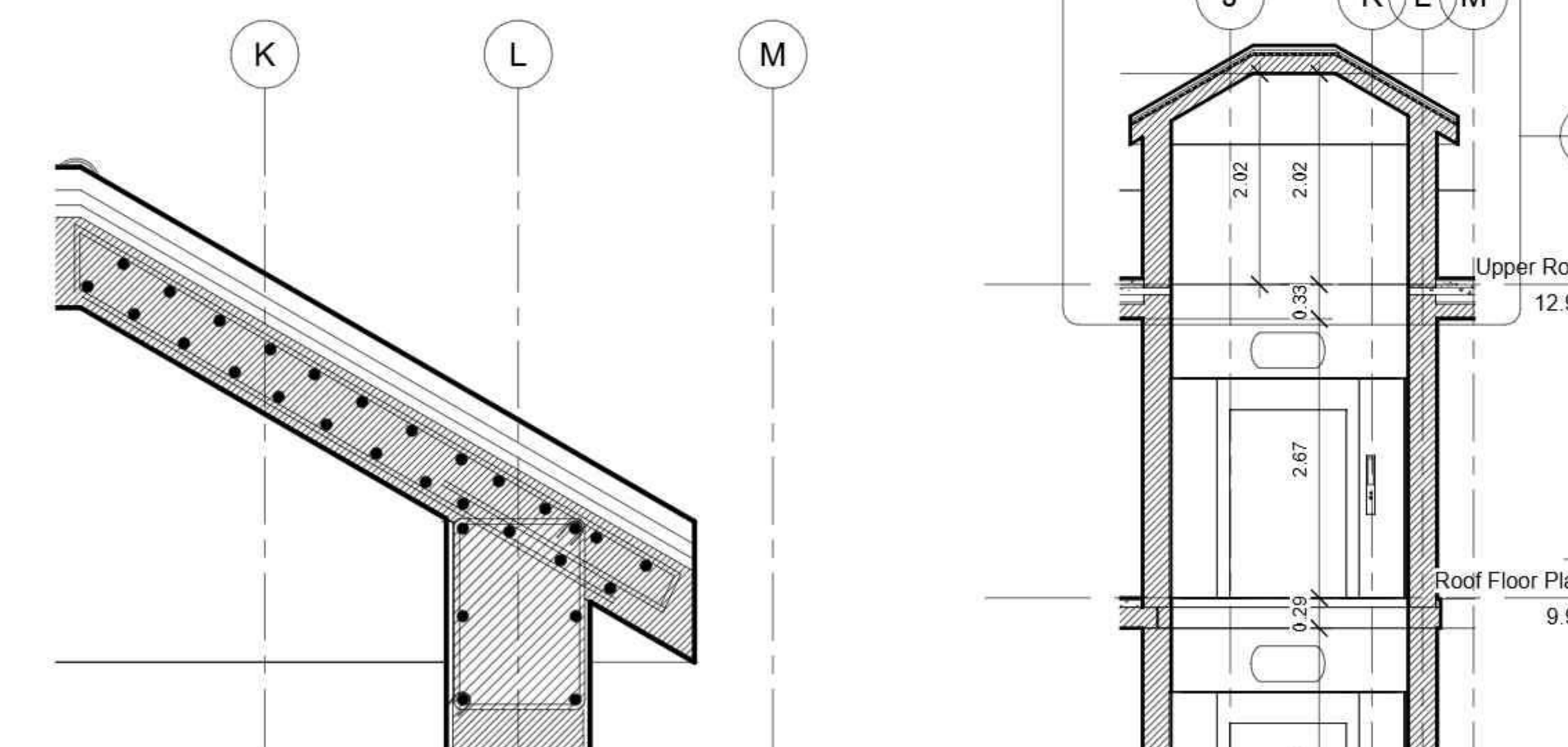
Pitched Roof Detail 1 : 20
