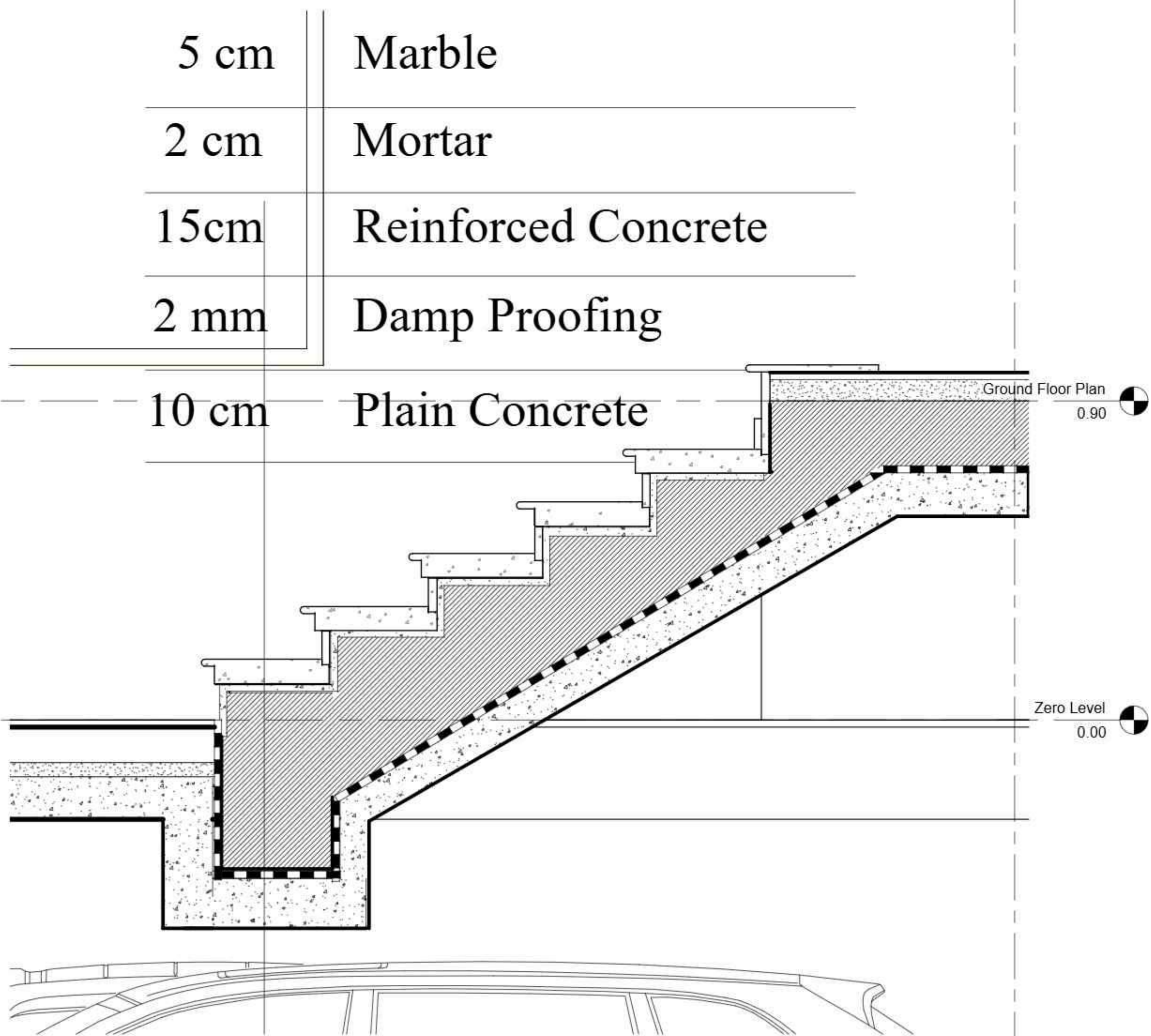
3 Entrance Wall Section - Callout 1 1:10
