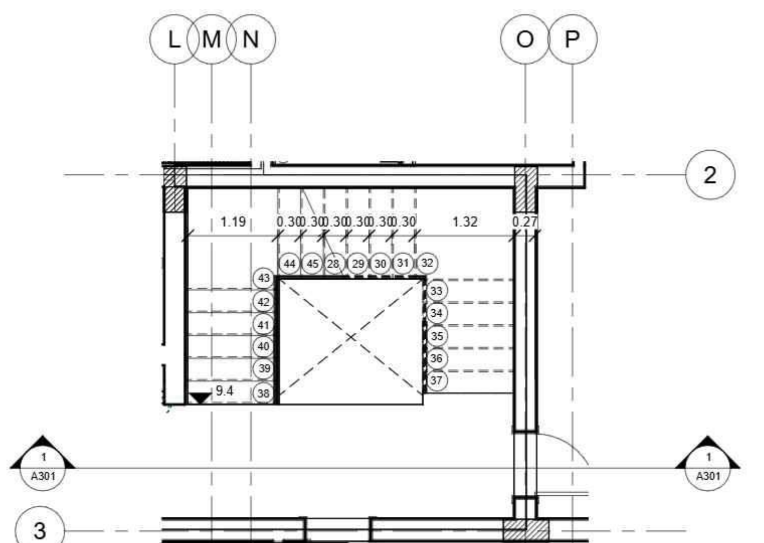
First Floor Plan - Callout 1 1 : 50
