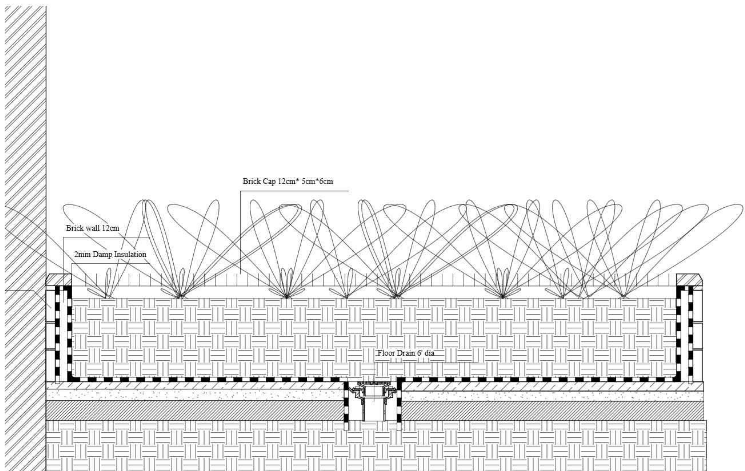
3 Flower Box Details 1 : 10
