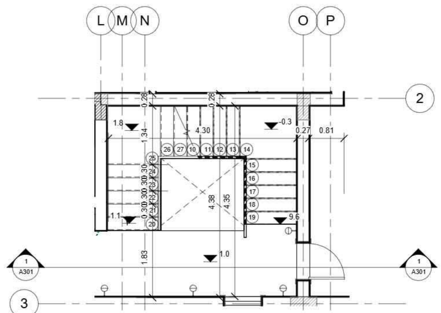
Ground Floor Plan - Callout 1 : 50
