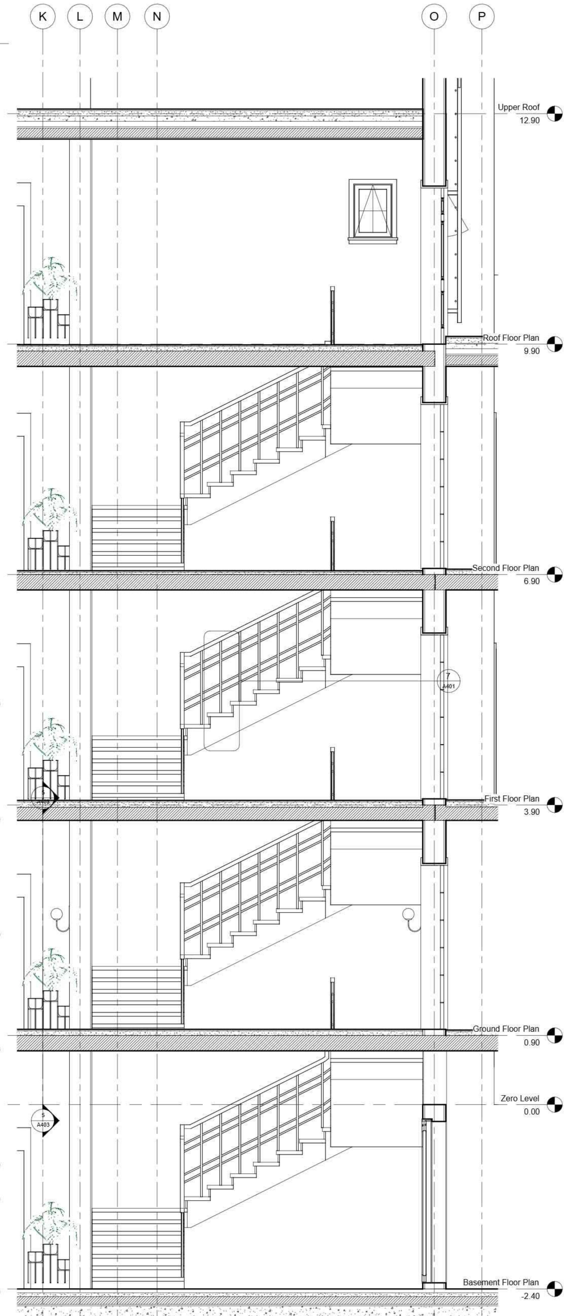
Marble Stairs Layers 1 : 20
