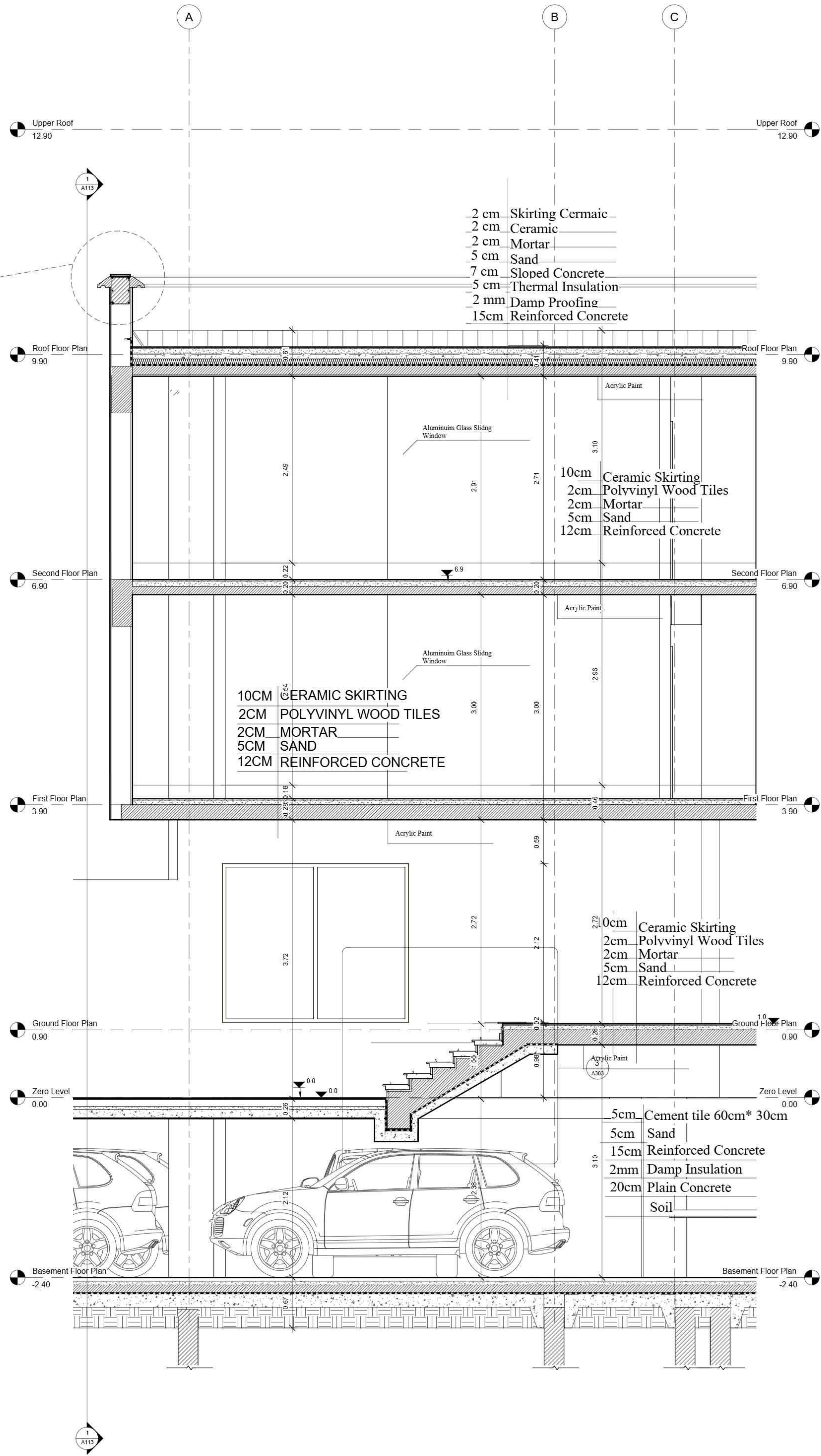
1 Entrance Wall Section 1:25
