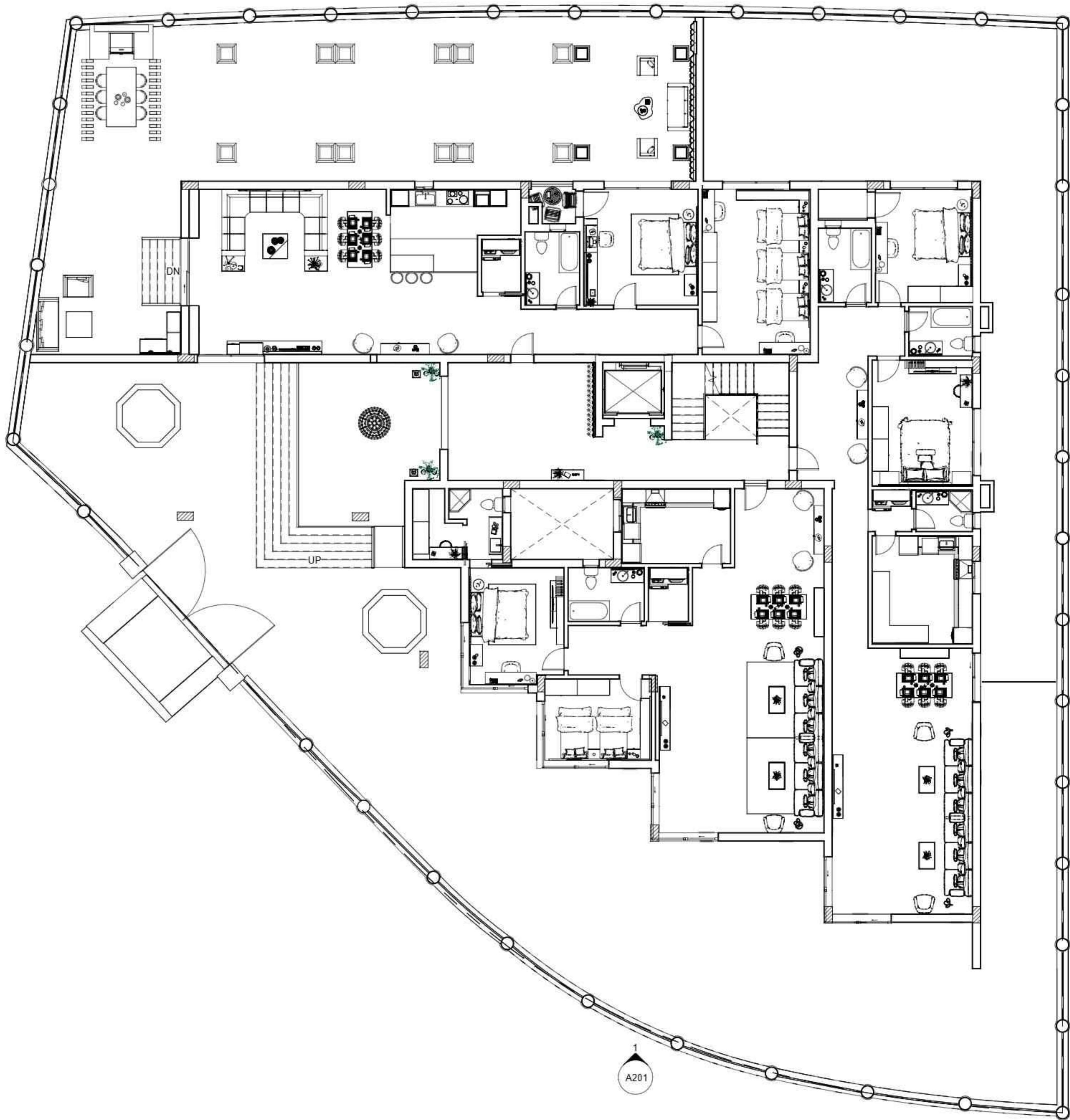
1 Ground Level Furnished 1 : 100
