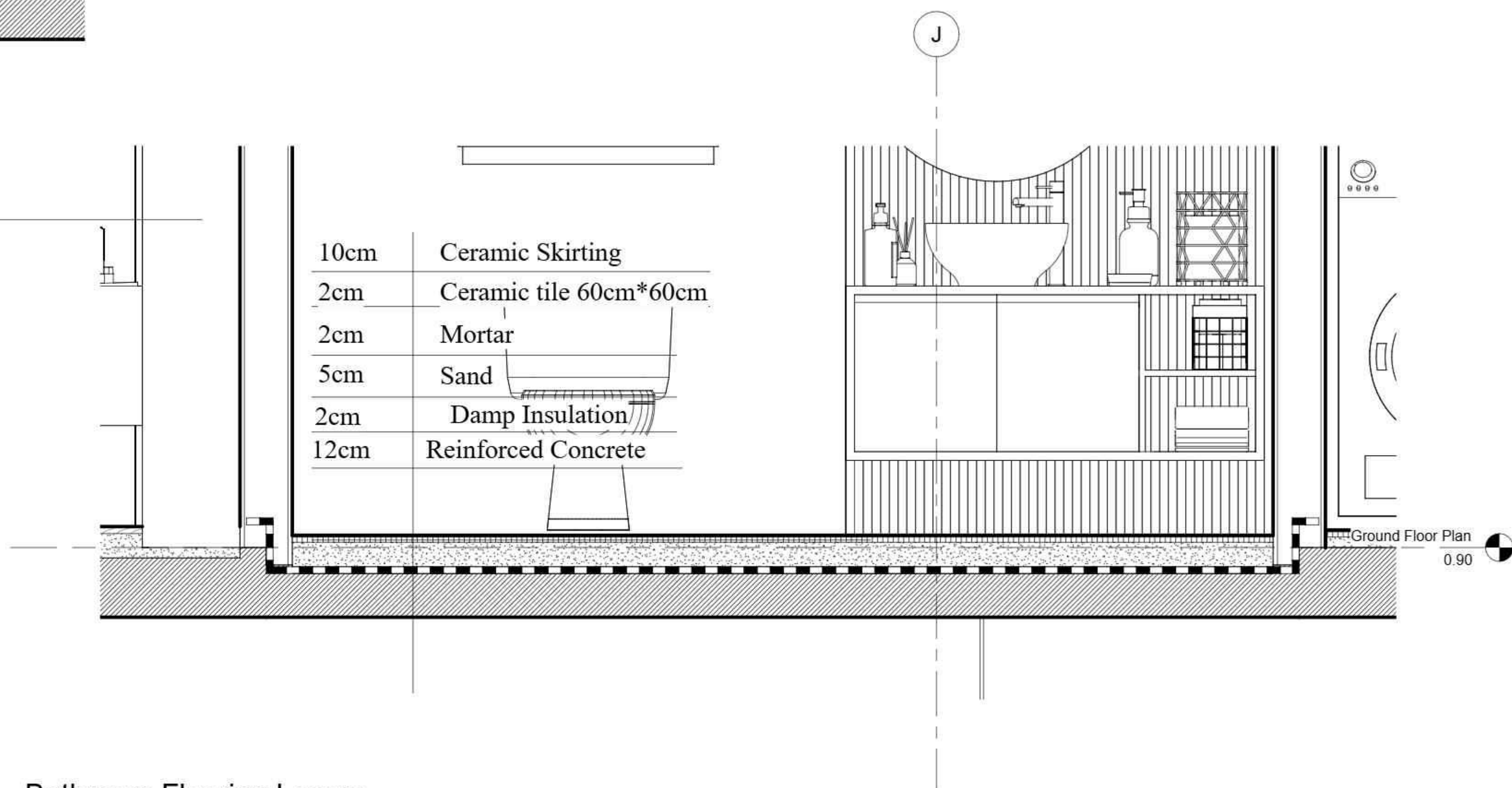
3 Bathroom Flooring Layers Copy 1 1 : 10
