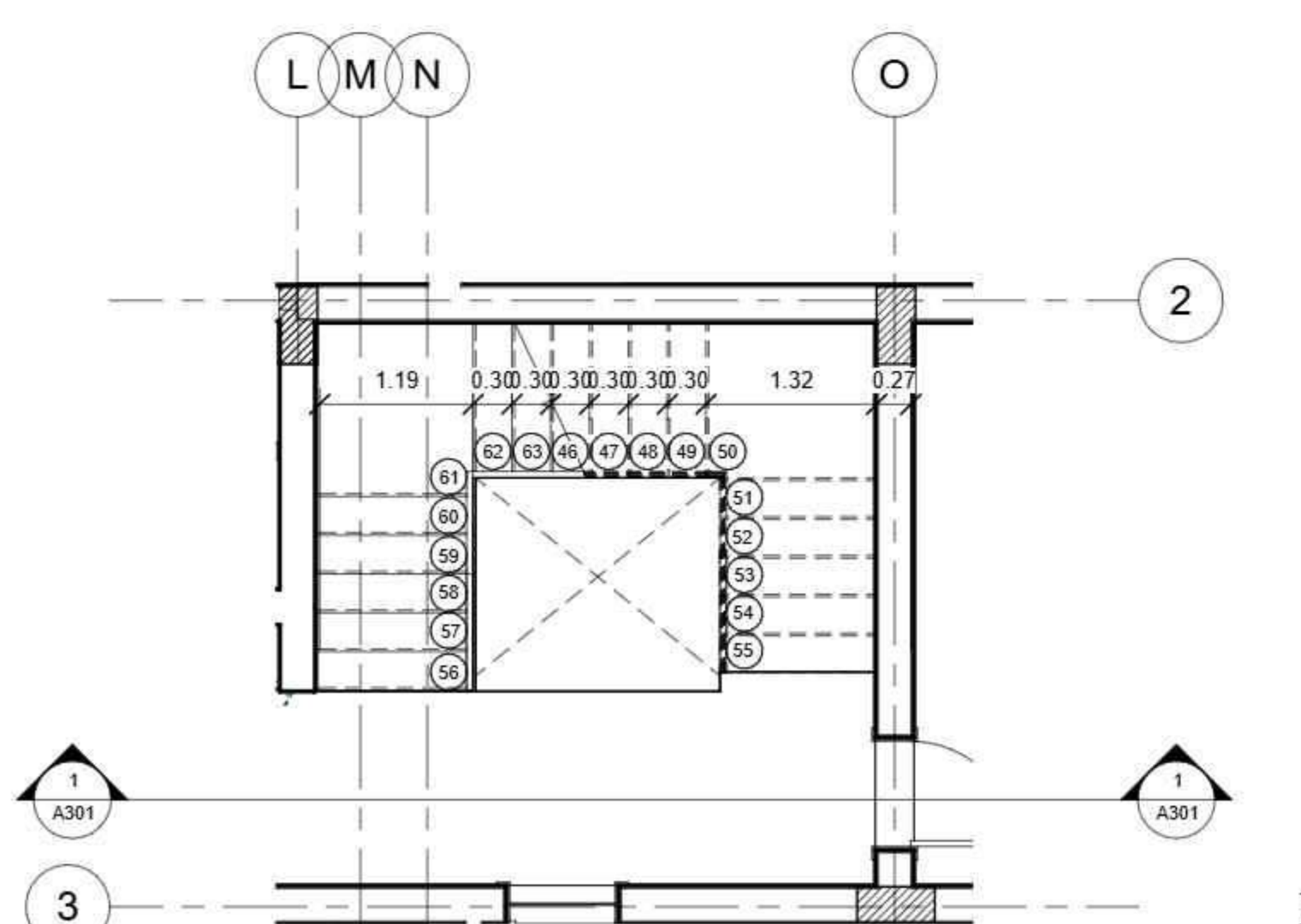
Second Floor Plan - Callout 1 : 50
