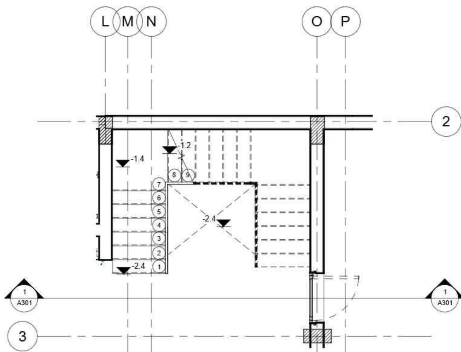
Basement Floor Plan - Callout 1 1 : 50
