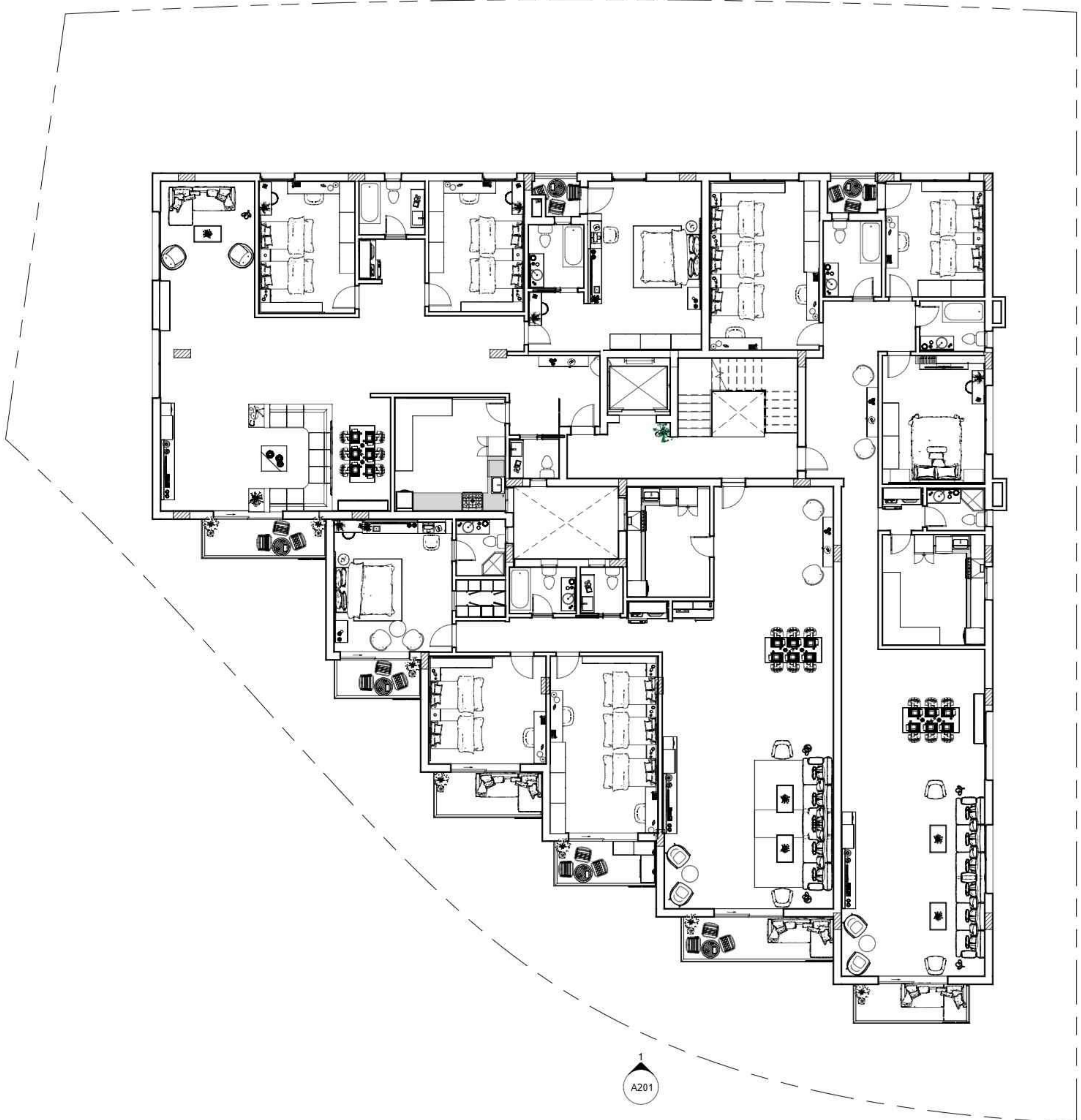
2 First Floor Furnished 1 : 100
