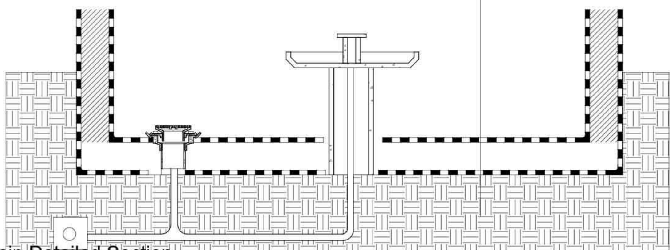
1 Fountain Detailed Section 1 : 10
