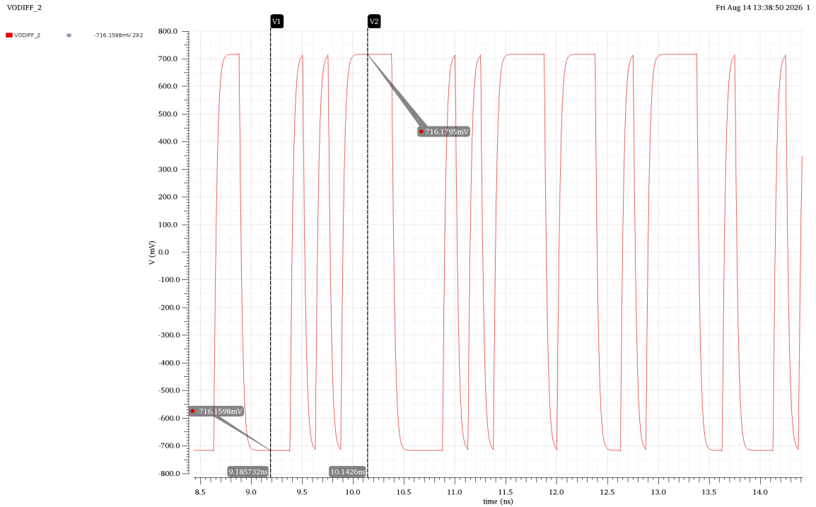
Figure 14: Transient response of the differential output of the optimized high-swing voltage-mode driver.
