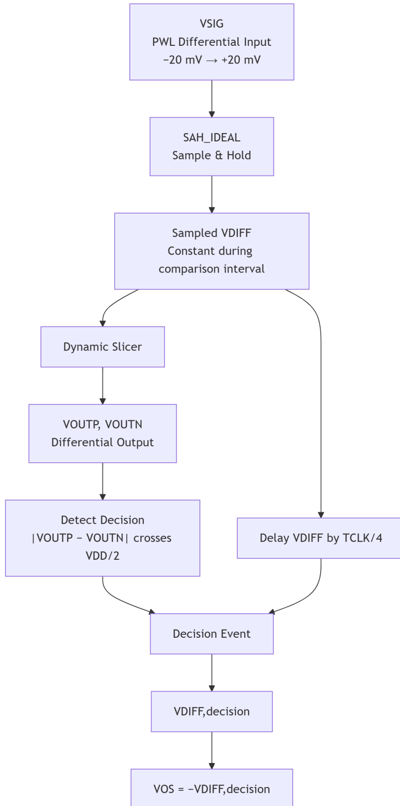
Figure 14: Flow of the input-referred offset voltage measurement.
