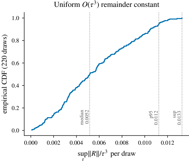
Fig. 9. Uniform remainder (arm ii): empirical CDF of the per-draw remainder constant \sup_\tau \|R\|/\tau^3 over 220 shape draws; the quoted 0.0133 is the supremum, not a typical value.
