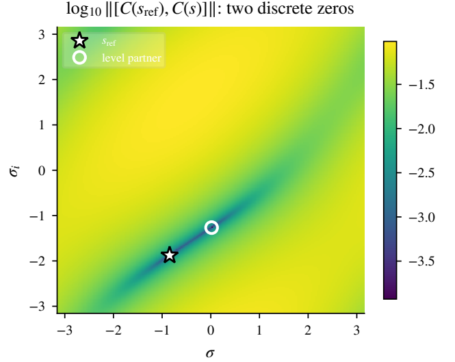
Fig. 7. The protected class, globally. \log_{10} \|[C(s_{\text{ref}}), C(s)]\| over the shape torus, with s_{\text{ref}} the first C15 pair’s first shape (star). An exhaustive basin-polished scan finds exactly two zeros: the reference and one isolated level partner (circle, 1.057 rad away) with C = C_{\text{ref}} — the discrete level set on which holonomy protection is exact at all orders.
