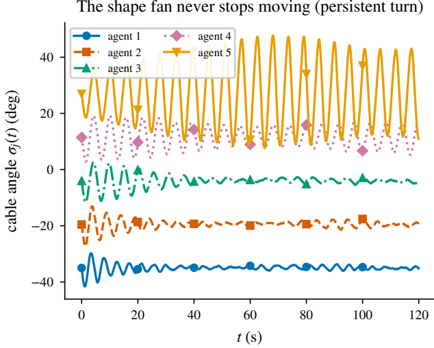
Fig. 2. The real cable-angle trajectories \sigma_j(t) from the reduced-plant run: the shape fan never stops moving under the persistent turn, so the lagged transports carry a nonzero twist and the floor is active.
