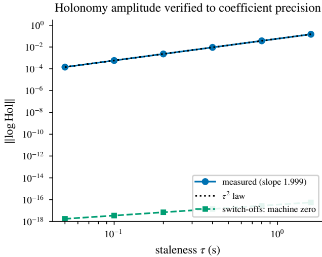
Fig. 13. Measured \|\text{Log Hol}\| vs. \tau (analytic shapes). Generic pair: fitted slope 1.999 over \tau \in [0.05, 1.6] s; the coefficient ratio \|\text{Log Hol}\|/\tau^2 \|[C_i, C_j]\| = 1.0000 at the smallest \tau . Switch-off arms ( s_i = s_j ; \eta = 0 ; \xi = 0 ) sit at machine zero ( \xi = 0 literally 0.0) — the effect dies exactly when the theorem requires it to.
