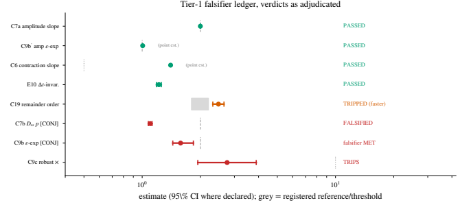
Fig. 14. The complete Tier-1 falsifier ledger, verdicts as registered. Green = passed; red = falsified / falsifier met ([CONJECTURAL] rows — measured slopes reported as measured, no law asserted); orange = tripped favorably (C19: the remainder vanishes faster than the registered second order). Grey dashes and bands are the registered references and thresholds; evidence file named per row.
