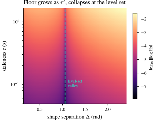
Fig. 6. The floor as a field: \log_{10} \|\log \text{Hol}\| over staleness \tau (vertical, log) and shape separation \Delta (horizontal, along a ray through the level-set partner). The amplitude grows as \tau^2 and collapses in a narrow valley at the level-set separation (dashed) — the growth law and the protected class in a single view.
