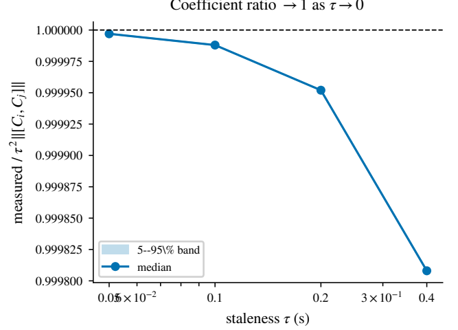
Fig. 10. Bound tightness: the measured/predicted ratio \|\text{Log Hol}\|/\tau^2 \|C_i, C_j\| rises to 1 as \tau \rightarrow 0 , the 5--95% band across 60 draws narrower than 2 \times 10^{-4} .
