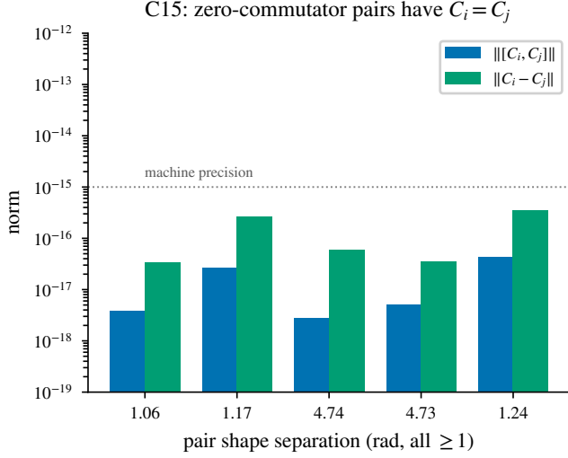
Fig. 12. Level-set protection (arm iv): the five zero-commutator pairs found at \geq 1 rad separation all satisfy C_i = C_j to 10^{-16} (both bars below machine precision) — the protected class is a level set, not just coincident shapes.
