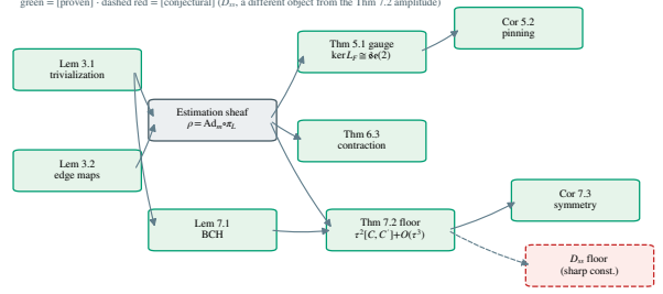
Fig. 3. Statement-dependency map and proof roadmap of the full theory, drawn with the companion’s numbering (the letter’s own results appear as Lem 3.1 = Lemma 1, Lem 7.1 = Lemma 2, Thm 7.2 = Theorem 1, Cor 7.3 = Corollary 1). Solid green = [PROVEN]: the floor chain is proved or sketched in this letter; the gauge/pinning/contraction branch is proved in the companion and shown for context only. Grey = the sheaf construction (definitions); dashed red = the [CONJECTURAL] stochastic steady-state object, deliberately shown outside the proved chain — it is the boundary discussed in Sec. V, not a dependency of the theorem.
