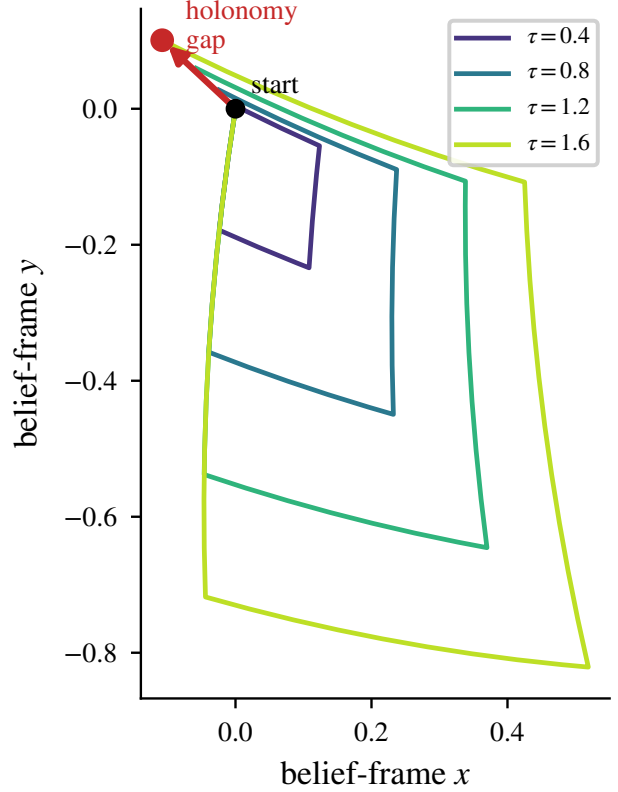
Fig. 4. Generic pair: the transported belief's trail is a closed walk that does not close. The red arrow is the holonomy gap for the largest \tau ; the nested loops grow with \tau \in \{0.4, 0.8, 1.2, 1.6\} . The visible failure-to-close is the disagreement a stale round trip injects.
