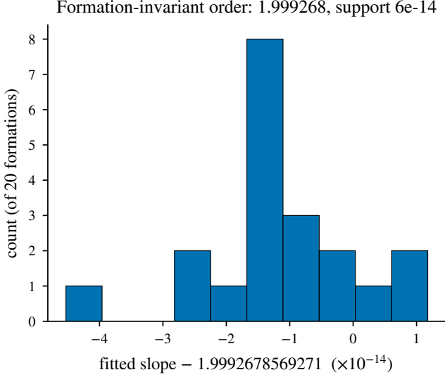
Fig. 8. Formation invariance (arm i): the 20 per-formation fitted slopes, in deviation units, span only 5.7 \times 10^{-14} around 1.9993 — the \tau^2 order is a structural constant.
