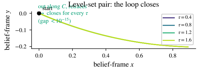
Fig. 5. Level-set pair ( C_i = C_j ): the walk goes out along the common generator and retraces exactly, returning to the start (gap < 10^{-15} ) at every \tau — exact protection at all orders.
