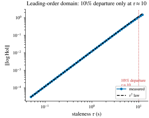
Fig. 11. Outside the leading-order domain: the measured amplitude departs from the \tau^2 law by 10% only at \tau \approx 10 — an order of magnitude beyond the operating grid ( \tau \leq 1.6 ), where the relative departure stays below 3.4 \times 10^{-3} . The theorem is a small- \tau statement and this is its measured boundary.
