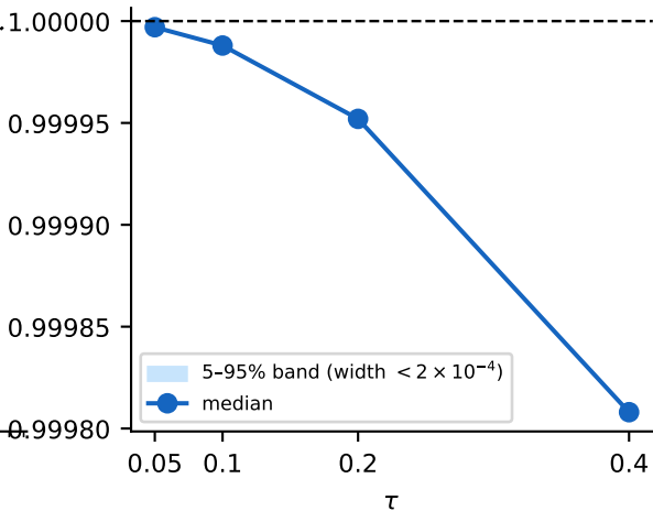
(b) the O(\tau^3) gap closes as \tau \rightarrow 0
