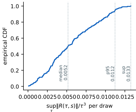
(a) remainder constant, 220 shape draws
