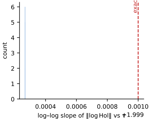
(b) fitted slope, 20 formations: 1.9993 \pm 1.2e-14
