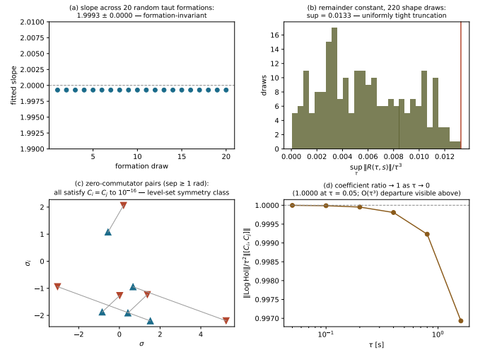
Fig. 7. Extension arms. (a) Slope across 20 random tau-t formations: 1.9993 \pm 0.0000 — formation-invariant. (b) Remainder constant over 220 draws: uniformly tight O(\tau^3) truncation. (c) Zero-commutator pairs at \geq 1 rad separation all satisfy C_i = C_j to 10^{-16} : the protected class is a level set. (d) Coefficient ratio \rightarrow 1 as \tau \rightarrow 0 .
