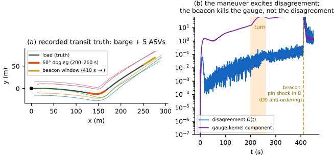
Fig. 4. The recorded 450s dogleg transit (from the committed hero_dogleg_series.npz ). (a) Truth: barge + 5 vessels, turn and beacon windows marked. (b) Disagreement D(t) vs. the gauge-kernel component: the maneuver excites the former; only the beacon kills the latter; the acquisition spike in D is the pin shock.
