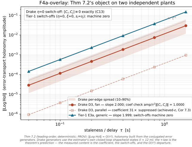
Fig. 8. Error-transport holonomy amplitude on both plants. Thm 7.2 (leading-order, deterministic): Tier-1 slope 1.999 with switch-offs at machine zero; Drake slope 2.000 with the m=2 coefficient check at 1.0000, the \eta=0 switch-off at machine zero, and the parallel class suppressing the coefficient 31 \times (achieved- \epsilon ; exact cancellation remains the Tier-1 machine-zero result).
