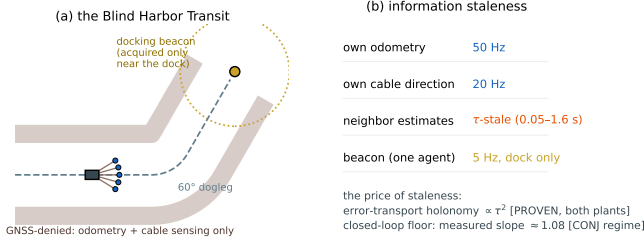
Fig. 1. (a) The Blind Harbor Transit: a GNSS-denied dogleg channel, one range-limited docking beacon at one vessel. (b) The information-staleness ladder: local sensing is fast, shared estimates are \tau -stale, absolute fixes exist only at the dock.
