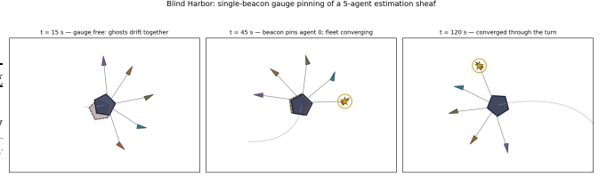
Fig. 3. Three phases of the GNSS-denied transit (supplementary video S2). Left: gauge free — the five ghost caissons (each agent’s own load estimate) drift coherently , overlapping each other while offset from truth. Middle: the beacon pins one agent; the fleet is mid-convergence. Right: converged through the turn. Single illustrative run, median- D_{ss} seed by the documented selection rule.
