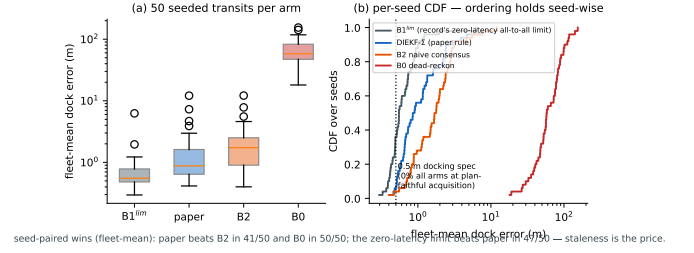
Fig. 6. The 50-transit scorecard at distribution level. (a) Fleet-mean dock error per arm (log scale — B0’s failure is two orders, not a tail). (b) Per-seed CDFs: the ordering holds seed-wise; the 0.5 m spec (dotted) is left of every support. Seed-paired win counts in the strip.
