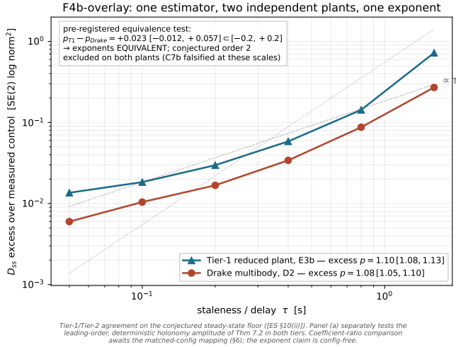
Fig. 9. Tier-1/Tier-2 agreement on the conjectured steady-state floor ([ES §10(ii)]). Panel (a) separately tests the leading-order, deterministic holonomy amplitude of Thm 7.2 in both tiers. With D_0 measured in situ by straight-tow controls, the fitted excess exponents are 1.101 [1.076, 1.125] (Tier-1) and 1.077 [1.054, 1.102] (Drake); the pre-registered equivalence test passes ( +0.023 [-0.012, +0.057] \subset [-0.2, 0.2] ) and the conjectured order 2 is excluded on both plants. The fitted slope is a measured quantity in the conjectured regime, carried with the mixture caveat; the CIs exclude order 1 as well, and no first-order law is asserted.
