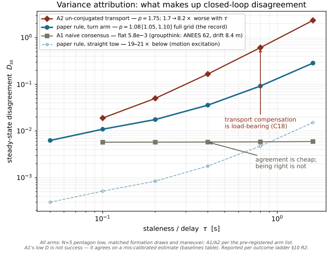
Fig. 10. All Drake arms on matched formation draws. Ablating the conjugated transport (A2) runs 1.7 \times \rightarrow 8.2 \times above the paper rule with growing \tau ; naive consensus (A1) holds disagreement flat and low—by grouphink (anchored ANEES 62, drift 8.4 m): agreement alone is never a virtue metric. The straight-tow control shows the motion excitation (19-21 \times at every \tau ).
