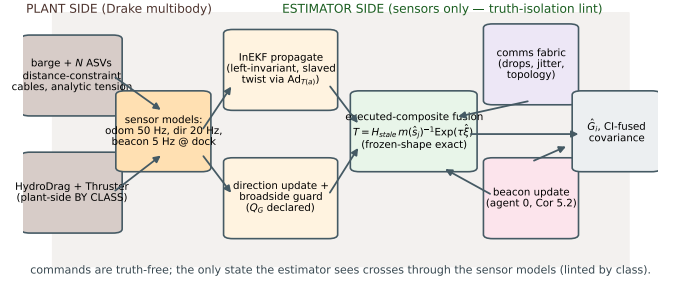
Fig. 2. DIEKF- \Sigma as executed, with the linted plant/estimator boundary. Per agent: invariant propagation through the slaved twist, direction updates with the broadside guard, executed-composite delayed fusion with CI covariance handling, and (one agent) the beacon channel.
