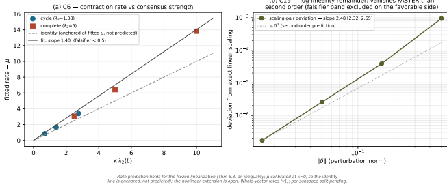
Fig. 13. Contraction in its own domain (frozen, unanchored); rate versus \kappa \lambda_2 across two topologies, slope 1.40 (falsifier < 0.5); \mu calibrated at \kappa = 0 , so the identity line is anchored, not predicted. The log-linearity remainder vanishes faster than the registered second order (2.48 [2.32, 2.65]; falsifier band excluded on the favorable side, reported as tripped with the corrected order).
