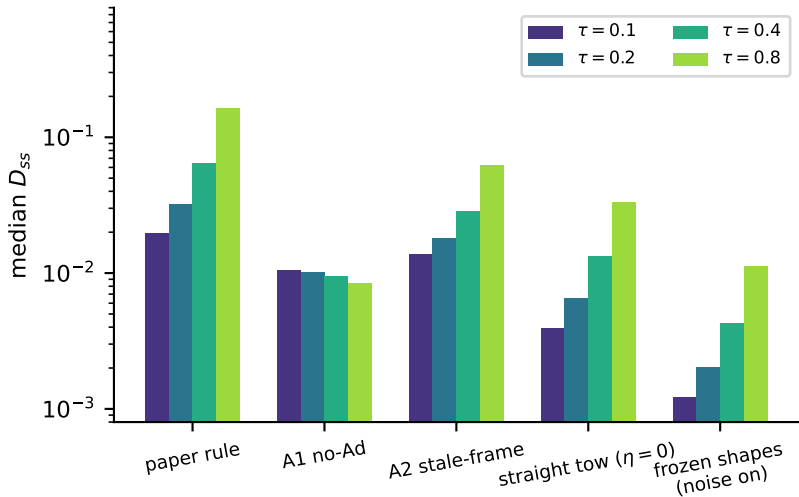
E3b arms — median D_{ss} [CONJ]. A1 below paper: the Tier-1 ordering inversion (C18) — D_{ss} never ranks rules
