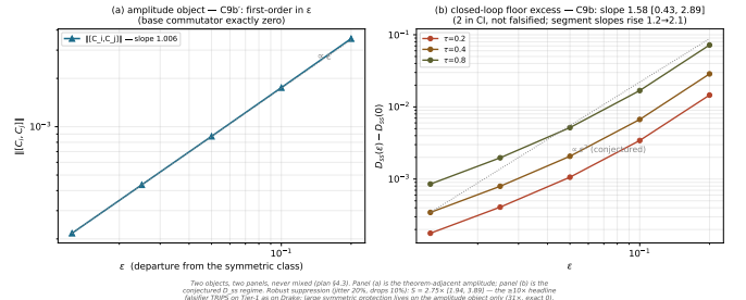
Fig. 9. F5: amplitude (a) and closed-loop floor (b) \epsilon -response, never mixed in one panel.
