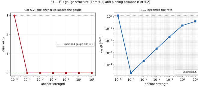
Fig. 3. Gauge spectrum: \dim \ker L_{\mathcal{F}} = 3 with the harmonic sections exactly the body-framed images of one common load-frame perturbation; one anchor removes the kernel.
