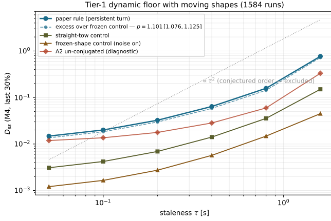
Fig. 6. Numerical evidence for the conjectured stochastic steady-state floor ((ES §10(ii))); Theorem 7.2 is leading-order and deterministic and is tested in panel F4a. Fitted excess exponent 1.101 [1.076, 1.125]: the conjectured order 2 is excluded (and so is 1); the frozen+noise-off regression reproduces the executed null ( D_{ss} \sim 10^{-30} ).
