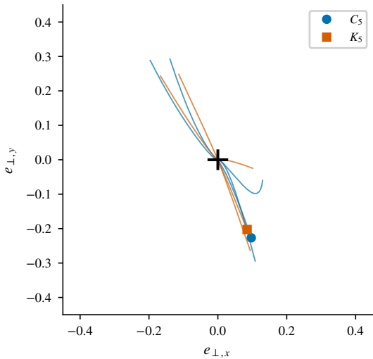
E2: gauge-complement error spirals to consensus
