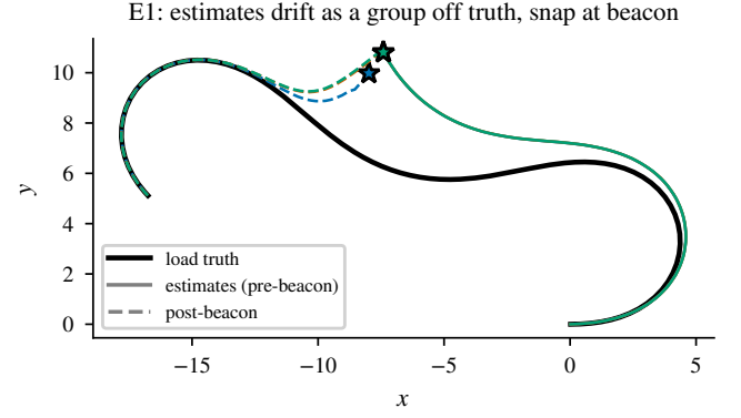
Fig. 4. The gauge phenomenon as trajectories: with no anchor the agents' load-pose estimates (colours) track each other but drift as a rigid group off the truth (black); at the beacon (stars) they snap back (dashed).
