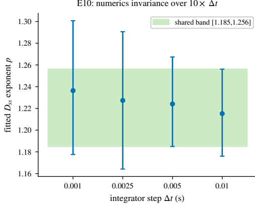
Fig. 19. E10: the fitted exponent across a 10\times range of integrator steps; all CIs share the green band [1.185, 1.256] .
