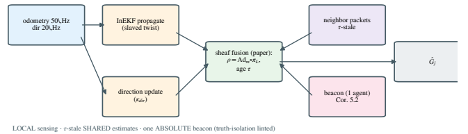
Fig. 2. The executed estimator pipeline and its information boundary: local sensing (odometry, cable direction), \tau -stale shared estimates transported through \rho = \text{Ad}_m \circ \pi_L with sheaf weights w_e , and at most one absolute anchor. Nothing else touches truth (lined).
