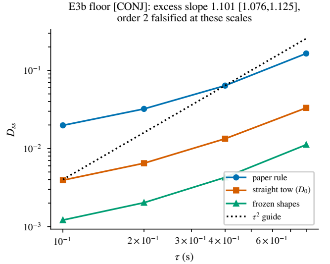
Fig. 9. Numerical evidence for the conjectured stochastic steady-state floor (IES §10(ii)); Theorem 7.2 is leading-order and deterministic and is tested in Fig. 6. Fitted excess exponent 1.101 [1.076, 1.125]: the conjectured order 2 is excluded (and so is 1); the frozen+noise-off regression reproduces the executed null ( D_{ss} \sim 10^{-30} ).
