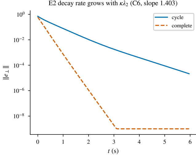
Fig. 18. The gauge-complement decay: its rate scales with \kappa\lambda_2 (C6, slope 1.403), faster on the more connected graph.
