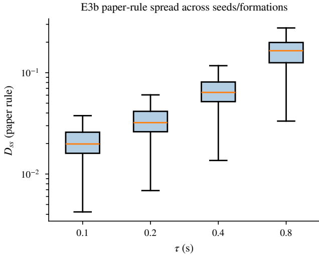
Fig. 11. Paper-rule D_{ss} spread across seeds and formations per \tau ([[CONJECTURAL] regime]).
