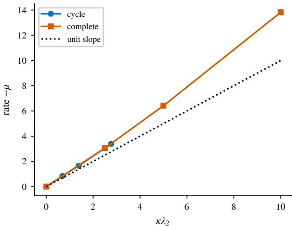
E2 contraction: rate \propto \kappa\lambda_2 (slope 1.403)
