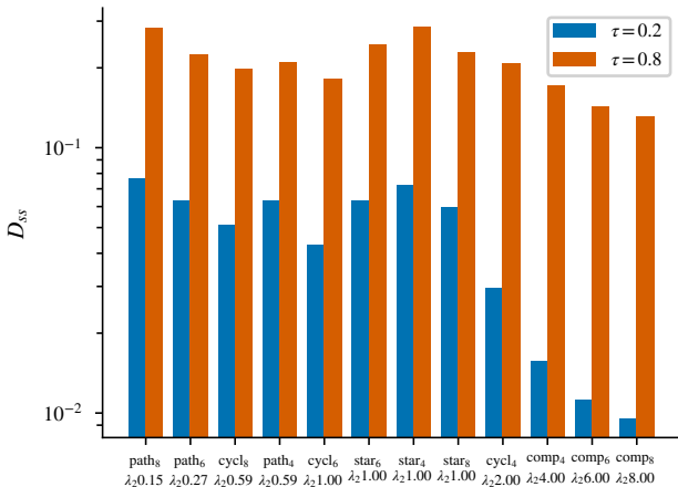
E6 (C10): connectivity suppresses the floor at moderate \tau
