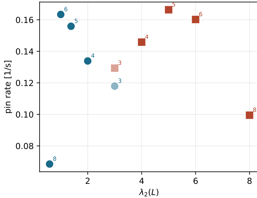
(b) gauge PIN rate vs \lambda_2 — Cor 5.2 observable Spearman +0.04: anchor-limited, NOT connectivity-limited
