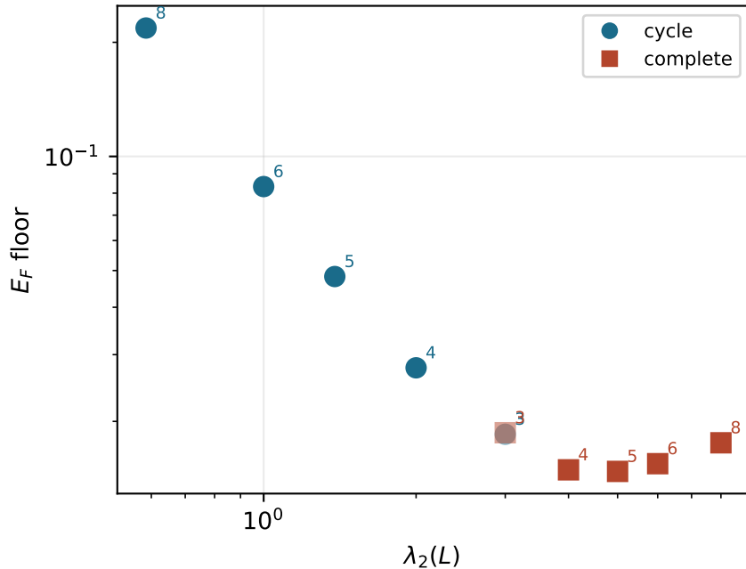
(a) pre-anchor floor vs \lambda_2 (cycles degrade with N ; complete flat)
