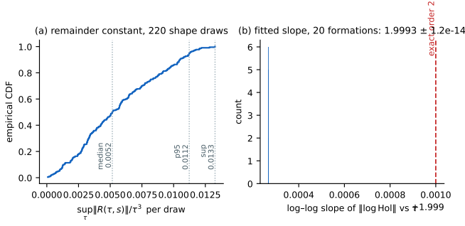
Fig. 4. Distributions behind the summary numbers. (a) Empirical CDF of the per-draw remainder constant \sup_{\tau} \|R\|/\tau^3 over 220 shape draws; the quoted 0.0133 is the supremum. (b) All 20 per-formation slopes: support width 3 \times 10^{-13} .
