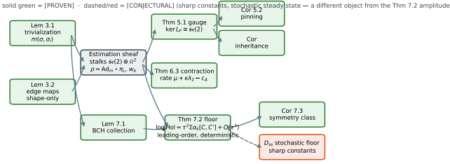
Fig. 2. Statement-dependency map and proof roadmap. Solid green = [PROVEN] (proved, with the proof or sketch in this letter); grey = the sheaf construction (definitions); dashed red = the [CONJECTURAL] stochastic steady-state object, deliberately shown outside the proved chain — it is the boundary discussed in Sec. V, not a dependency of the theorem.
