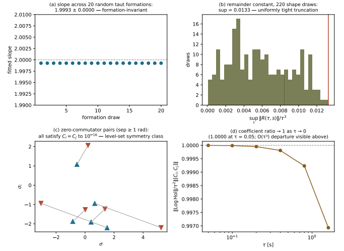
Fig. 7. Extension arms. (a) Slope across 20 random tau-t formations: 1.9993 \pm 0.0000 — formation-invariant. (b) Remainder constant over 220 draws: uniformly tight O(\tau^3) truncation. (c) Zero-commutator pairs at \geq 1 rad separation all satisfy C_i = C_j to 10^{-16} : the protected class is a level set. (d) Coefficient ratio \rightarrow 1 as \tau \rightarrow 0 .
