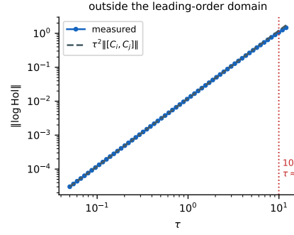
Fig. 6. Outside the leading-order domain: the measured amplitude departs from the \tau^2 law by 10% only at \tau \approx 10 — an order of magnitude beyond the operating grid ( \tau \leq 1.6 ), where the relative departure stays below 3.4 \times 10^{-3} . The theorem is a small- \tau statement and this is its measured boundary.
