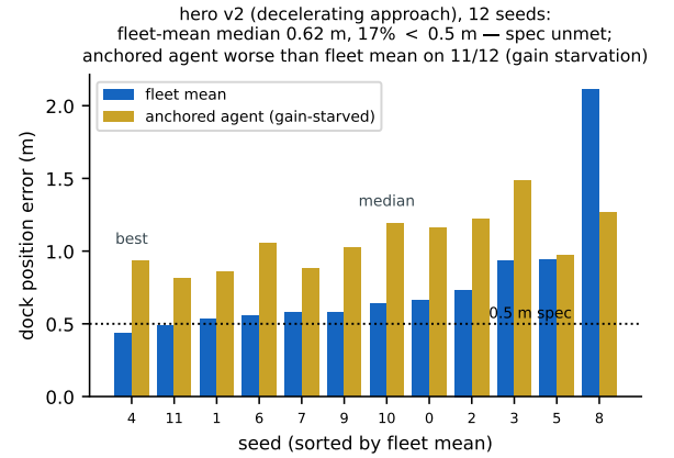
Fig. 7. Hero v2 (decelerating approach), all 12 seeds sorted: fleet-mean vs. anchored-agent dock error. Median 0.62 m, 17% under spec — improvement without sufficiency; the anchored agent is worse than the fleet mean on 11/12 seeds (gain starvation); best/median/worst marked, worst shown.
