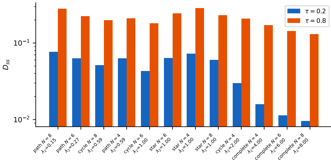
C10 (exploratory): connectivity suppresses the floor at moderate \tau ; benefit collapses at high \tau
