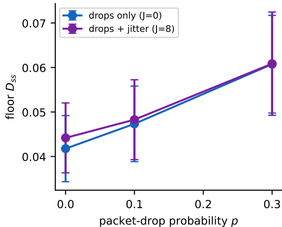
(a) D10(b): graceful — +13% @ p=0.1 , +45% @ p=0.3 ; ANEES in-gate (4.23, 130 s)
