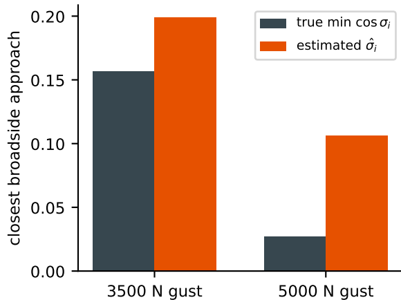
(b) D10(c): \hat{\sigma}_i LAGS true broadside — guard unexercised (ON \equiv OFF)
