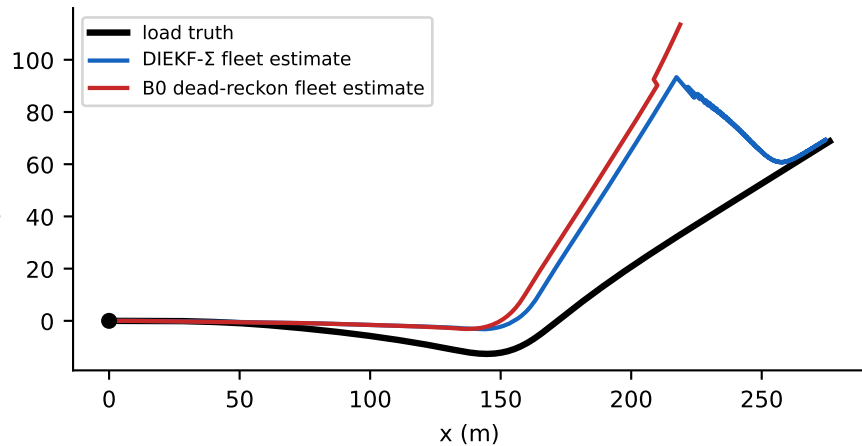
(a) fleet load-pose estimate tracks vs truth
