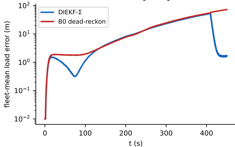
(b) the sheaf fusion holds the load; dead-reckoning diverges
