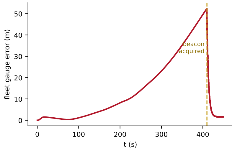
(b) the group drift (gauge error) grows under GNSS denial; one anchor collapses it
