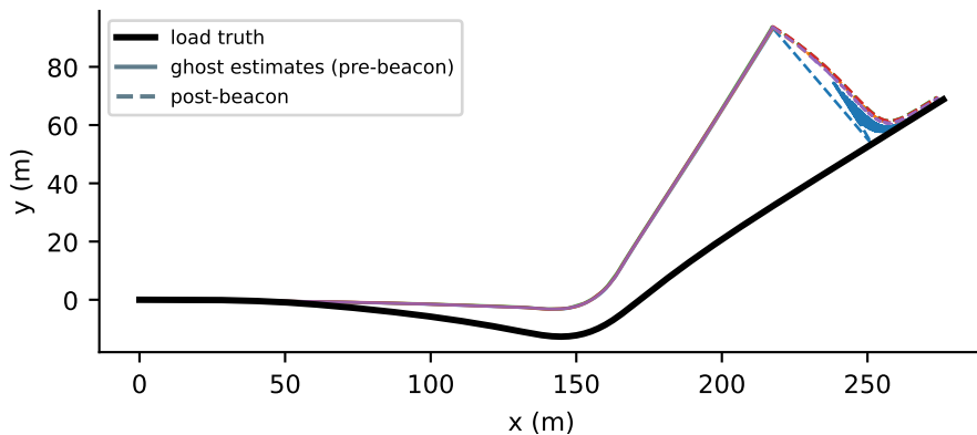
(a) five ghost load-pose estimates drift as a group off the truth, then collapse at beacon
