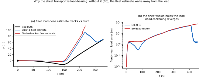
Fig. 12. Why the sheaf transport is load-bearing. (a) Fleet load-pose estimate tracks: the DIEKF- \Sigma (blue) follows the truth and is pinned at the beacon, while B0 dead-reckoning (red) walks away. (b) Fleet-mean load error: the sheaf fusion propagates the single anchor to the whole fleet at the dock, collapsing to \sim 1 m; dead-reckoning cannot, and diverges (matching the 1.6 m vs. 67 m scorecard means).
