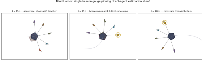
Fig. 5. Three phases of the GNSS-denied transit (supplementary video S2). Left: gauge free — the five ghost caissons (each agent’s own load estimate) drift coherently , overlapping each other while offset from truth. Middle: the beacon pins one agent; the fleet is mid-convergence. Right: converged through the turn. Single illustrative run, median- D_{ss} seed by the documented selection rule.
