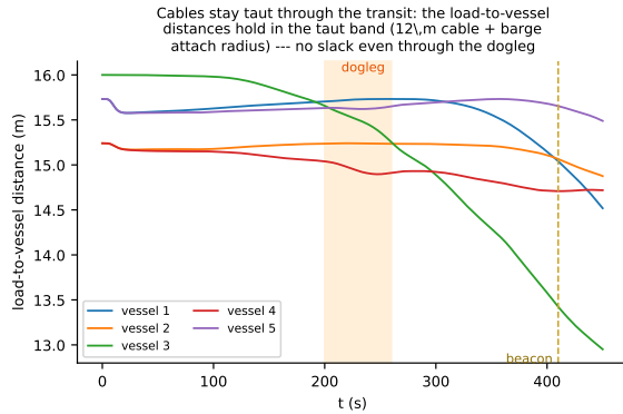
Fig. 3. Constraint satisfaction through the transit: the load-to-vessel distances hold in the taut band (12m cable plus the barge attachment radius) — the distance-constraint cables never go slack, even through the dogleg.
