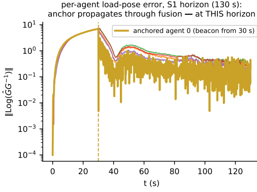
Fig. 8. Per-agent load-pose error at the 130s calibration horizon (recorded hero_series.npz ): the beacon at agent 0 (gold, from 30s) propagates through fusion to the whole fleet — at this horizon. The 450s failure of this picture is the gain-starvation finding of Fig. 10.
