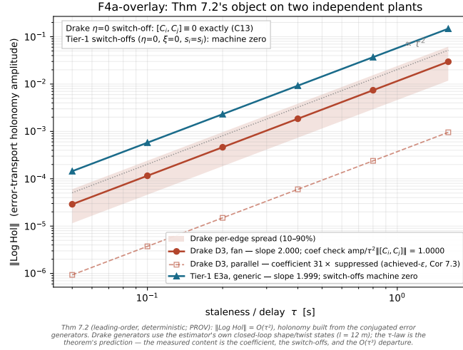
Fig. 13. Error-transport holonomy amplitude on both plants. Thm 7.2 (leading-order, deterministic): Tier-1 slope 1.999 with switch-offs at machine zero; Drake slope 2.000 with the m=2 coefficient check at 1.0000, the \eta=0 switch-off at machine zero, and the parallel class suppressing the coefficient 31\times (achieved- \epsilon ; exact cancellation remains the Tier-1 machine-zero result).
