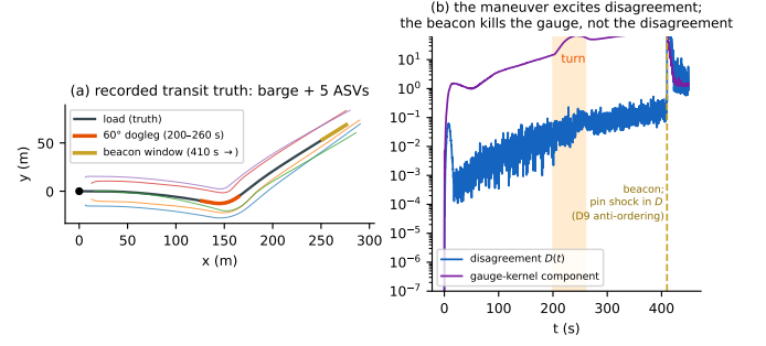
Fig. 6. The recorded 450 s dogleg transit (from the committed hero_dogleg_series.npz ). (a) Truth: barge + 5 vessels, turn and beacon windows marked. (b) Disagreement D(t) vs. the gauge-kernel component: the maneuver excites the former; only the beacon kills the latter; the acquisition spike in D is the pin shock.
