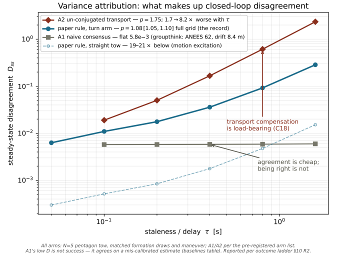
Fig. 15. All Drake arms on matched formation draws. Ablating the conjugated transport (A2) runs 1.7\times \rightarrow 8.2\times above the paper rule with growing \tau ; naive consensus (A1) holds disagreement flat and low—by groupthink (anchored ANEES 62, drift 8.4 m; baselines cell, 130 s horizon): agreement alone is never a virtue metric. The straight-tow control shows the motion excitation (19–21 \times at every \tau ).
