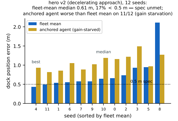
Fig. 10. Hero v2 (decelerating approach), all 12 seeds sorted: fleet-mean vs. anchored-agent dock error. Median 0.61 m, 17% under spec — improvement without sufficiency; the anchored agent is worse than the fleet mean on 11/12 seeds (gain starvation); best/median/worst marked, worst shown.
