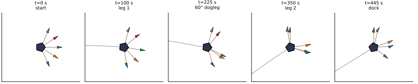
Fig. 2. The recorded transit, five ordered snapshots: the pentagon barge towed by five ASVs on cables (coloured triangles) through the GNSS-denied dogleg, with the load's ground-truth trail behind it. From the committed multibody run (seed 3).
