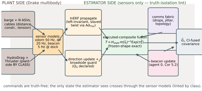
Fig. 4. DIEKF- \Sigma as executed, with the linted plant/estimator boundary. Per agent: invariant propagation through the slaved twist, direction updates with the broadside guard, executed-composite delayed fusion with CI covariance handling, and (one agent) the beacon channel.
