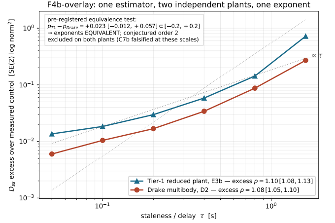
Fig. 14. Tier-1/Tier-2 agreement on the conjectured steady-state floor ([ES §10(ii)]). The leading-order, deterministic holonomy amplitude of Thm 7.2 is tested separately in Fig. 13. With D_0 measured in situ by straight-tow controls, the fitted excess exponents are 1.101 [1.076, 1.125] (Tier-1) and 1.077 [1.054, 1.102] (Drake); the pre-registered equivalence test passes ( +0.023 [-0.012, +0.057] \subset [-0.2, 0.2] ) and the conjectured order 2 is excluded on both plants. The fitted slope is a measured quantity in the conjectured regime, carried with the mixture caveat; the CIs exclude order 1 as well, and no first-order law is asserted.
