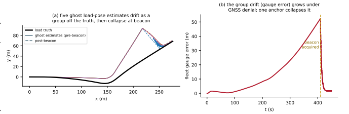
Fig. 7. Cor. 5.2 in the closed loop, spatially. (a) The five agents’ load-pose estimates (colours) stay a tight, consistent fleet but drift as a group off the truth (black) through GNSS denial, then collapse toward it once the dock beacon is acquired (solid \rightarrow dashed). (b) The fleet gauge error grows to tens of metres and is killed by the single anchor. From the committed hero_ghost_tracks.npz (seed 3).
