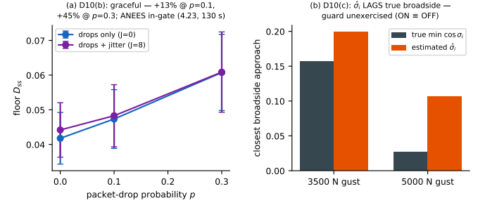
Fig. 19. D10 robustness characterization (outside class \mathcal{P} ). (a) Floor vs. packet-drop probability, drops-only and drops+jitter arms (8 seeds each; mean \pm sd): graceful, no red flags; anchored ANEES in-gate at p=0.3 at the 130 s horizon. (b) Why the broadside guard never fired: \hat{\sigma}_i lags true broadside across the reachable gust envelope — ON \equiv OFF, reported as a null with its mechanism.
