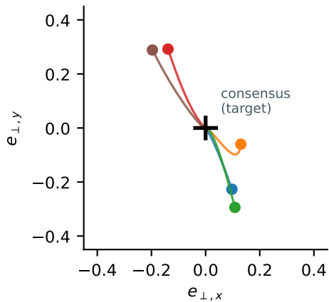
(a) C_5 cycle ( \lambda_2=1.38 )
