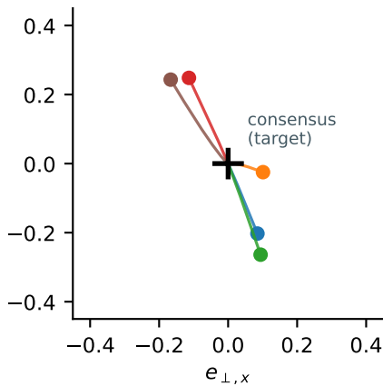
(b) K_5 complete ( \lambda_2=5 )
