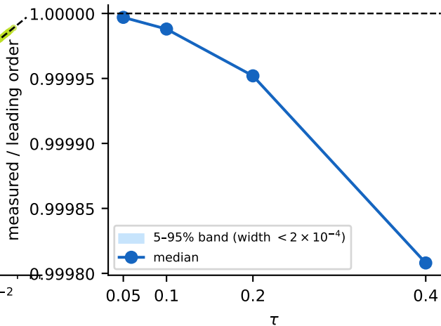
(b) the O(\tau^3) gap closes as \tau \rightarrow 0
