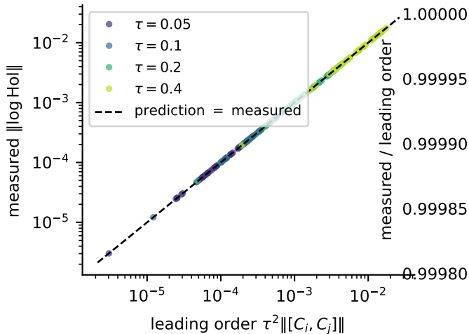
(a) tightness, 60 draws \times 4 \tau
