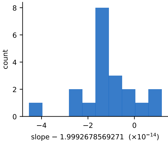
(b) fitted slope, 20 formations: 1.999268 support width 5.7e-14; offset from 2 is the finite- \tau fit
