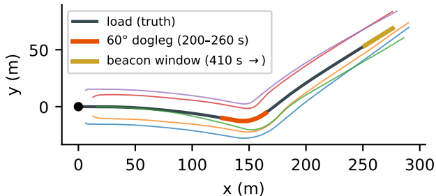
(a) recorded transit truth: barge + 5 ASVs
