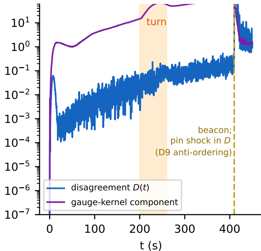
(b) the maneuver excites disagreement; the beacon kills the gauge, not the disagreement
