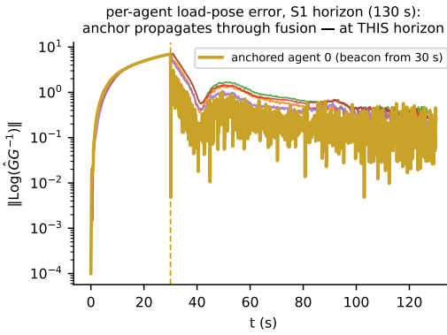
Fig. 5. Per-agent load-pose error at the 130s calibration horizon (recorded hero_series.npz ): the beacon at agent 0 (gold, from 30 s) propagates through fusion to the whole fleet — at this horizon. The 450s failure of this picture is the gain-starvation finding of Fig. 7.
