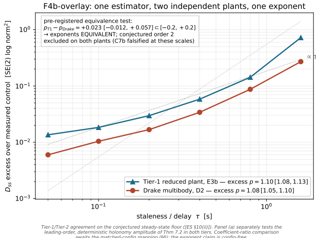
Fig. 9. Tier-1/Tier-2 agreement on the conjectured steady-state floor ([ES §10(ii)]). The leading-order, deterministic holonomy amplitude of Thm 7.2 is tested separately in Fig. 8. With D_0 measured in situ by straight-tow controls, the fitted excess exponents are 1.101 [1.076, 1.125] (Tier-1) and 1.077 [1.054, 1.102] (Drake); the pre-registered equivalence test passes ( +0.023 [-0.012, +0.057] \subset [-0.2, 0.2] ) and the conjectured order 2 is excluded on both plants. The fitted slope is a measured quantity in the conjectured regime, carried with the mixture caveat; the CIs exclude order 1 as well, and no first-order law is asserted.
