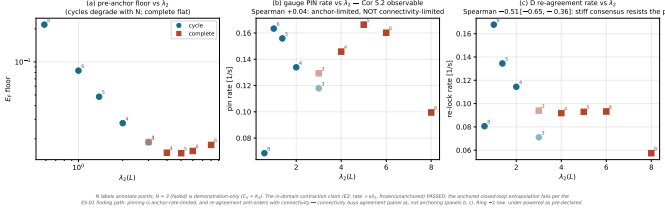
Fig. 12. Connectivity buys agreement, not anchoring. The pre-anchor floor improves with \lambda_2 (a); single-anchor pinning is anchor-rate-limited (b, Spearman +0.04); re-agreement around the pin anti -orders with connectivity (c, -0.51 [-0.65, -0.36] ). With the in-domain contraction claim verified (Fig. 13), this is the pre-registered ES-01 finding path, reported as such.
