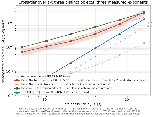
Fig. 16. The epistemic spine in one overlay: three distinct objects, three measured exponents — Tier-1 \|\text{Log Hol}\| ( p = 2.00 , the theorem’s object, [PROVEN]); the Drake round-trip transport defect ( p = 1.00 , estimate-mismatch dominated); and the Drake closed-loop D_{ss} ( p = 1.08 [1.05, 1.10], [CONJECTURAL] regime, D_0 measured by the straight-tow control 19–21 \times below). Never conflated.
