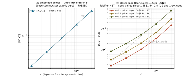
Two objects, two panels, never mixed (p4.3). Panel (a) is the theorem-adjacent amplitude; panel (b) is the conjectured D_0 regime under the ADJUDICATED seed paired estimator (the unpaired C1 is under-powered and adjudicates nothing; segment slopes rise 1.2 \rightarrow 2.1 — a linear-quadratic mixture the registered single-power model mis-specifies). Robust suppression (after 20%, drops 10%): 2.75 \times [1.94, 3.89] ratio of arm means — the \approx 10 \times falsifier TRIPS; large symmetric protection lives on the amplitude object only (31 \times Drake, exact 0 Tier-1).
