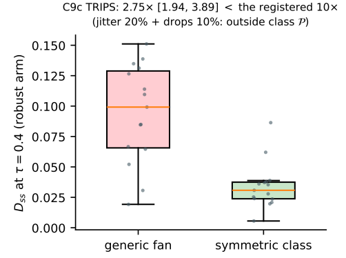
Fig. 8. The C9c trip at run level: generic vs. symmetric-class D_{ss} under 20% jitter + 10% drops (outside class \mathcal{P} ). Median ratio 2.75 \times [1.94, 3.89] — protection persists but falls an order short of the registered 10\times .
