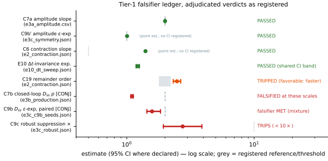
Fig. 14. The complete Tier-1 falsifier ledger, verdicts as adjudicated: green passed, red falsified/met ([CONJECTURAL] rows — measured slopes reported as measured), orange tripped favorably. Grey marks the registered references; the evidence record is named per row.
