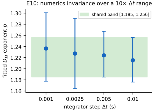
Fig. 11. E10: the fitted exponent across a 10\times range of integrator steps; all CIs share the green band [1.185, 1.256] .
