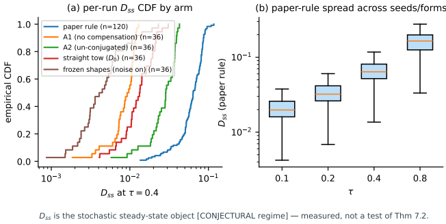
Fig. 7. Behind the fitted exponent: (a) per-run D_{ss} CDFs by arm at \tau = 0.4 (1584-run production record); (b) paper-rule spread across seeds/formations per \tau . D_{ss} is the stochastic steady-state object [[CONJECTURAL] regime] — measured, not a test of Thm. 7.2.
