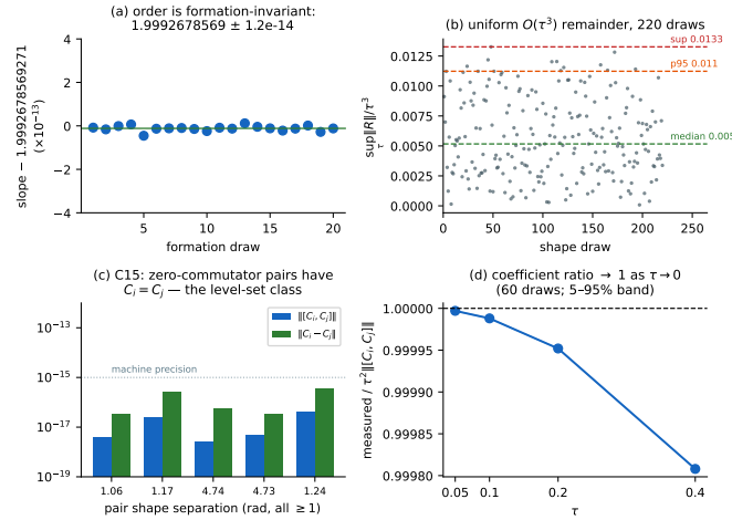
Fig. 5. E3a extension arms: formation-invariant order; uniform O(\tau^3) remainder; the level-set symmetry class; coefficient ratio \rightarrow 1 .
