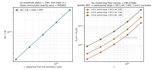
Two objects, two panels, never mixed (plan §4.3). Panel (a) is the theorem-adjacent amplitude; panel (b) is the conjectured D_{ss} regime under the ADJUDICATED seed-paired estimator (the unpaired CI is under-powered and adjudicates nothing; segment slopes rise 2.2 \sim 2.7 — a linear-quadratic measure the registered single-power model mis-specified). Robust suppression (jitter 20%, drops 10%): 2.75 \times [1.94, 3.89] ratio of arm means — the \approx 10\times falsifier TRIPS, large symmetric protection lives on the amplitude object only (33 \times Drake, exact 0 Tier-1).
