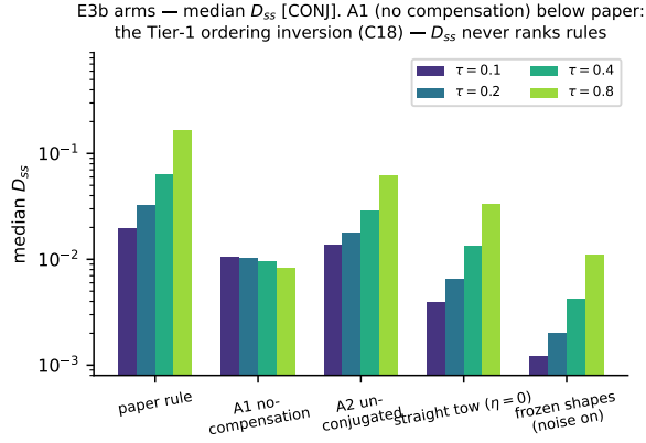
Fig. 13. E3b transport-rule and control arms, median D_{ss} by staleness [[CONJECTURAL] object]. The Tier-1 A1-below-paper inversion is shown, not smoothed: D_{ss} is a disagreement metric and never ranks rules — ranking is done on the companion’s truth-referenced metrics. The noise-off frozen null ( D_{ss} \sim 10^{-30} ) lies 27 orders below the axis and is reported in the table.
