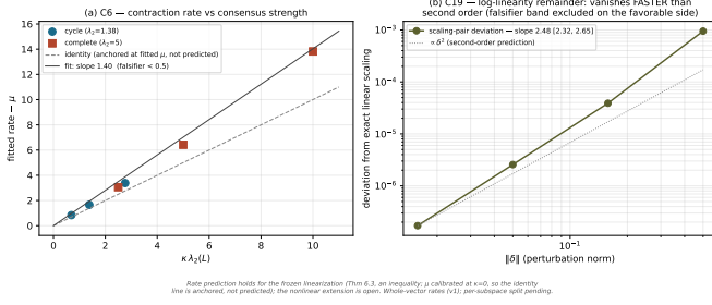
Fig. 10. F8: rate versus \kappa\lambda_2 across two topologies, slope 1.40 (falsifier < 0.5 ); \mu calibrated at \kappa = 0 , so the identity line is anchored, not predicted; the nonlinear extension is open.
