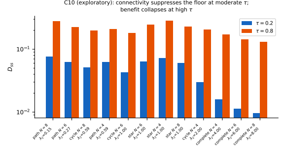
Fig. 12. E6 (exploratory, C10): floor vs. topology \times N ordered by \lambda_2 , at moderate ( \tau=0.2 ) and high ( \tau=0.8 ) staleness. Connectivity suppresses the floor 5\times at moderate \tau ; the benefit collapses at high \tau .
