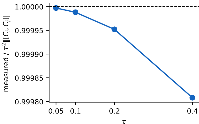
(d) coefficient ratio \rightarrow 1 as \tau \rightarrow 0 (60 draws; 5-95% band)
