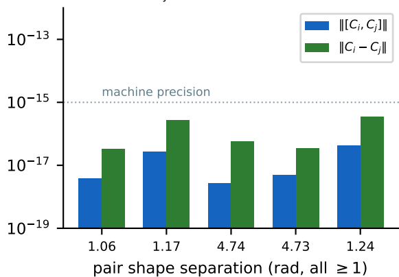
(c) C15: zero-commutator pairs have C_i = C_j — the level-set class
