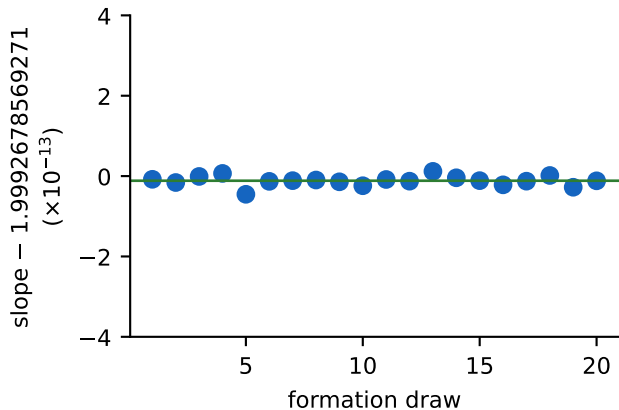
(a) order is formation-invariant: 1.9992678569 \pm 1.2\text{e-}14
