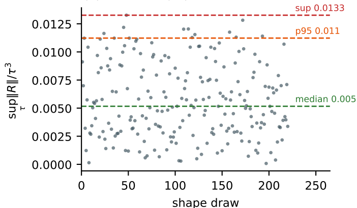
(b) uniform O(\tau^3) remainder, 220 draws
