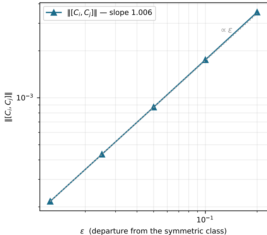
(a) amplitude object — C9b': first-order in \varepsilon (base commutator exactly zero) — PASSED
