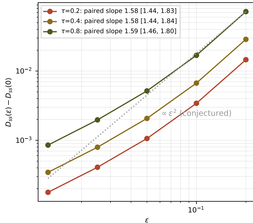
(b) closed-loop floor excess — C9b [CONJ]: falsifier MET — seed-paired slope 1.58 [1.44, 1.84], 2 and 1 excluded
