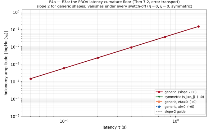
Fig. 1. Measured \|\text{Log Hol}\| vs. \tau (analytic shapes). Generic pair: fitted slope 1.999 over \tau \in [0.05, 1.6] s; the coefficient ratio \|\text{Log Hol}\|/\tau^2 \|[C_i, C_j]\| = 1.0000 at the smallest \tau . Switch-off arms ( s_i=s_j ; \eta=0 ; \xi=0 ) sit at machine zero ( \xi=0 literally 0.0) — the effect dies exactly when the theorem requires it to.
