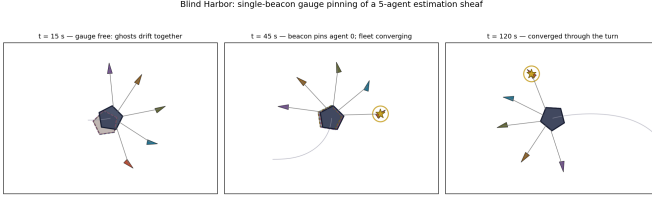
Fig. 1. Three phases of the GNSS-denied transit (supplementary video S2). Left: gauge free — the five ghost caissons (each agent’s own load estimate) drift coherently , overlapping each other while offset from truth. Middle: the beacon pins one agent; the fleet is mid-convergence. Right: converged through the turn. Single illustrative run, median- D_{ss} seed by the documented selection rule.
