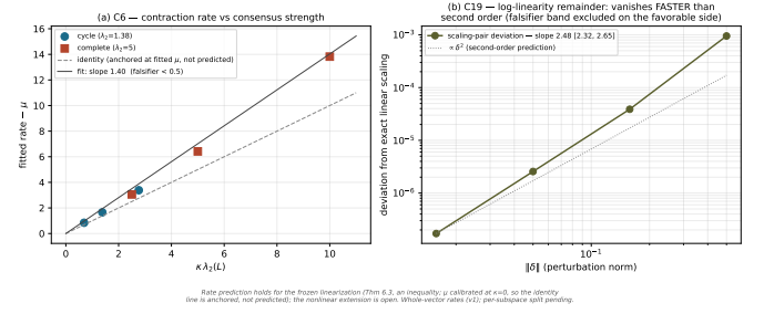
Fig. 7. Contraction in its own domain (frozen, unanchored): rate versus \kappa\lambda_2 across two topologies, slope 1.40 (falsifier < 0.5 ); \mu calibrated at \kappa = 0 , so the identity line is anchored, not predicted. The log-linearity remainder vanishes faster than the registered second order (2.48 [2.32, 2.65]; falsifier band excluded on the favorable side, reported as tripped with the corrected order).
