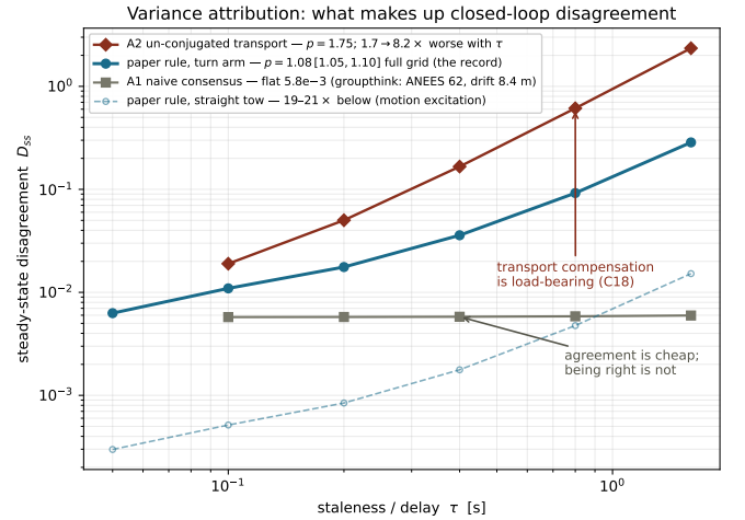
Fig. 4. All Drake arms on matched formation draws. Ablating the conjugated transport (A2) runs 1.7\times \rightarrow 8.2\times above the paper rule with growing \tau ; naive consensus (A1) holds disagreement flat and low—by groupthink (anchored ANEES 62, drift 8.4 m): agreement alone is never a virtue metric. The straight-tow control shows the motion excitation ( 19\text{--}21\times at every \tau ).
