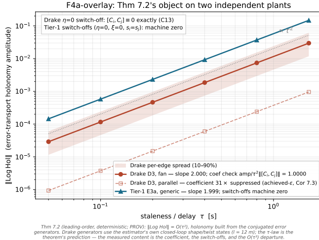
Fig. 2. Error-transport holonomy amplitude on both plants. Thm 7.2 (leading-order, deterministic): Tier-1 slope 1.999 with switch-offs at machine zero; Drake slope 2.000 with the m=2 coefficient check at 1.0000, the \eta=0 switch-off at machine zero, and the parallel class suppressing the coefficient 31\times (achieved- \varepsilon ; exact cancellation remains the Tier-1 machine-zero result).
