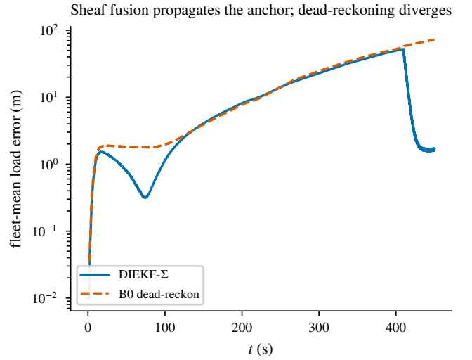
Fig. 18. Fleet-mean load error: the sheaf fusion propagates the single anchor to the whole fleet at the dock, collapsing to \sim 1 m; dead-reckoning cannot, and diverges (matching the 1.6 vs. 67 m scorecard means).
