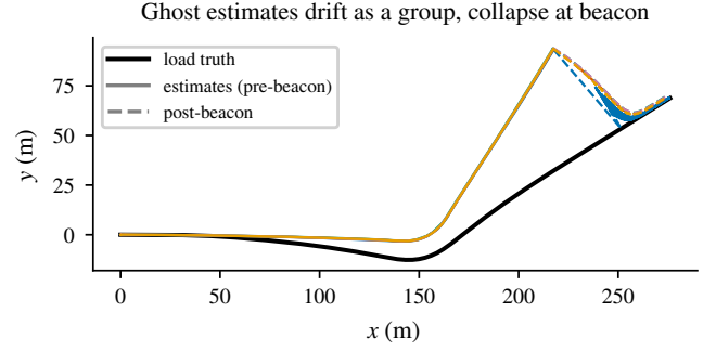
Fig. 9. Cor. 1 in the closed loop, spatially: the five agents' load-pose estimates (colours) stay a tight, consistent fleet but drift as a group off the truth (black) through GNSS denial, then collapse toward it once the dock beacon is acquired (solid \rightarrow dashed). From the committed hero_ghost_tracks.npz (seed 3).
