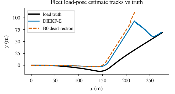
Fig. 17. Why the sheaf transport is load-bearing: fleet load-pose estimate tracks. The DIEKF- \Sigma (blue) follows the truth and is pinned at the beacon; B0 dead-reckoning (red) walks away.
