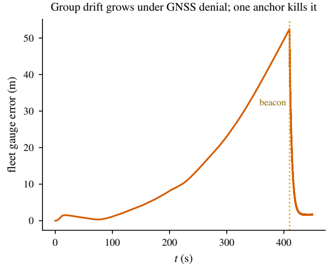
Fig. 10. The fleet gauge error (mean estimate vs. truth) grows to tens of metres under GNSS denial and is killed by the single dock anchor.
