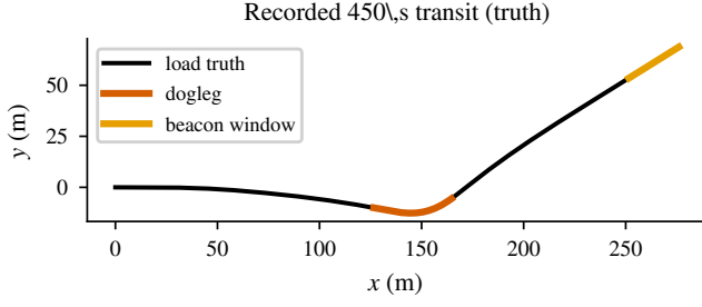
Fig. 7. The recorded 450s dogleg transit truth (from the committed hero_dogleg_series.npz ): barge trajectory with the turn and beacon windows marked.
