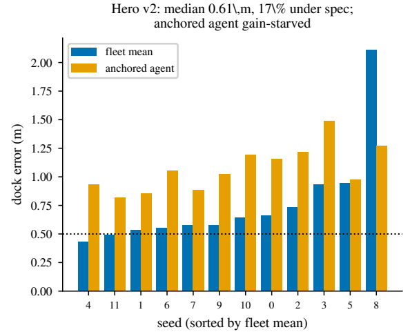
Fig. 14. Hero v2 (decelerating approach), all 12 seeds sorted: fleet-mean vs. anchored-agent dock error. Median 0.61m, 17% under spec — improvement without sufficiency; the anchored agent is worse than the fleet mean on 11/12 seeds (gain starvation); best/median/worst marked, worst shown.
