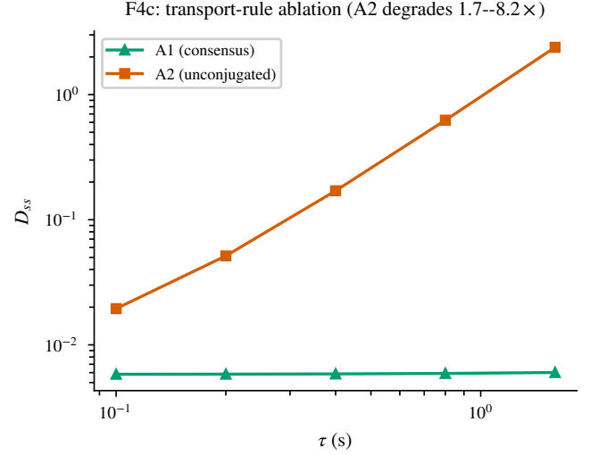
Fig. 21. All Drake arms on matched formation draws. Ablating the conjugated transport (A2) runs 1.7\times \rightarrow 8.2\times above the paper rule with growing \tau ; naive consensus (A1) holds disagreement flat and low—by groupthink (anchored ANEES 62 vs. the paper rule's 3.6, and drift 8.4 m vs. dead-reckoning's 1.9 m — the 17\times and 4.4\times of the abstract; baselines cell, 130 s horizon); agreement alone is never a virtue metric. The straight-tow control shows the motion excitation ( 19\text{--}21\times at every \tau ).
