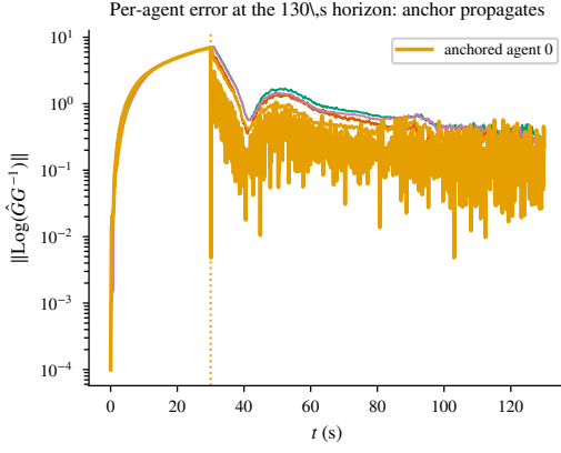
Fig. 11. Per-agent load-pose error at the 130s calibration horizon (recorded hero_series.npz ): the beacon at agent 0 (gold, from 30s) propagates through fusion to the whole fleet — at this horizon. The 450s failure of this picture is the gain-starvation finding of Fig. 14.
