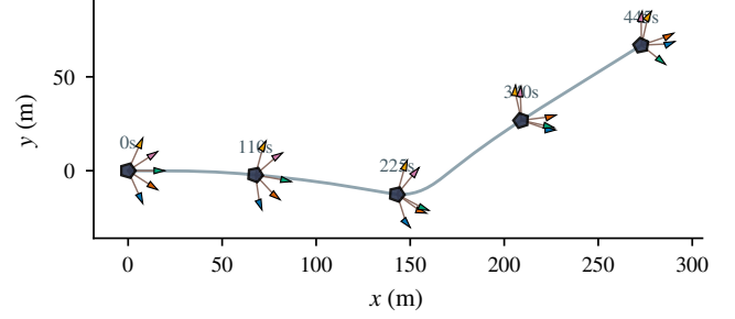
Recorded transit: barge + 5 ASVs through the dogleg
