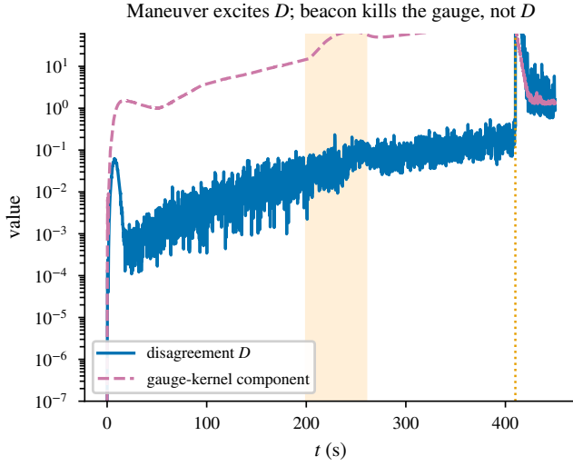
Fig. 8. Disagreement D(t) vs. the gauge-kernel component along the same transit: the maneuver excites the former; only the beacon kills the latter; the acquisition spike in D is the pin shock.
