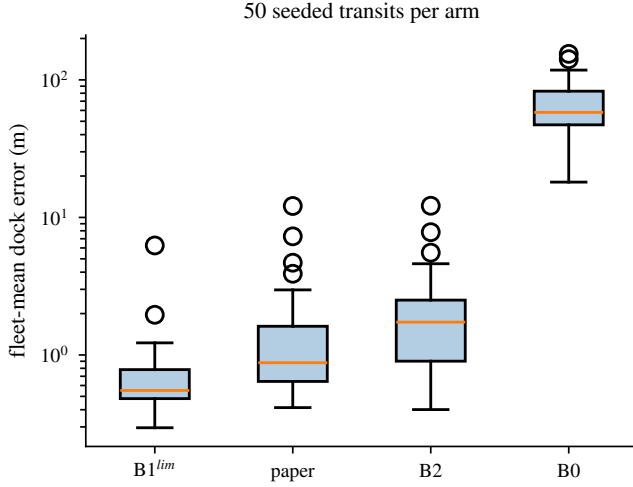
Fig. 12. The 50-transit scorecard: fleet-mean dock error per arm (log scale — B0's failure is two orders, not a tail).
