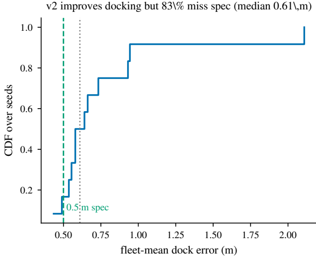
Fig. 16. Across seeds, the decelerating approach (v2) improves the fleet-mean dock error (median 0.61 m) but 83% of seeds still miss the 0.5 m spec — the approach geometry, not the estimator, binds.
