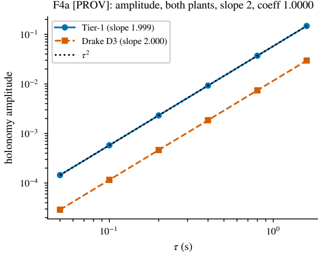
Fig. 19. Error-transport holonomy amplitude on both plants. Thm 3 (leading-order, deterministic): Tier-1 slope 1.999 with switch-offs at machine zero; Drake slope 2.000 with the m=2 coefficient check at 1.0000, the \eta=0 switch-off at machine zero, and the parallel class suppressing the coefficient 31\times (achieved- \varepsilon ; exact cancellation remains the Tier-1 machine-zero result).
