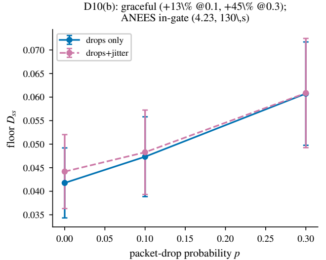
Fig. 26. D10(b) robustness (outside class \mathcal{P} ): floor vs. packet-drop probability, drops-only and drops+jitter arms (8 seeds each; mean \pm sd) — graceful, no red flags; anchored ANEES in-gate at p=0.3 at the 130 s horizon.
