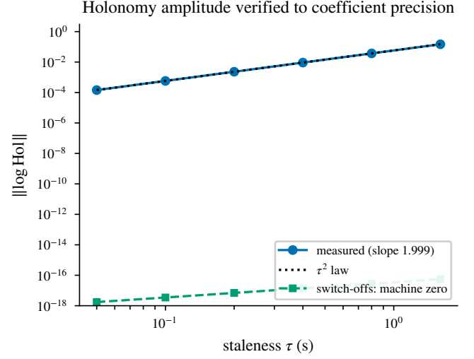
Fig. 13. Measured \|\text{Log Hol}\| vs. \tau (analytic shapes). Generic pair: fitted slope 1.999 over \tau \in [0.05, 1.6] s; the coefficient ratio \|\text{Log Hol}\|/\tau^2\| [C_i, C_j]\| = 1.0000 at the smallest \tau . Switch-off arms ( s_i = s_j ; \eta = 0 ; \xi = 0 ) sit at machine zero ( \xi = 0 literally 0.0) — the effect dies exactly when the theorem requires it to.
