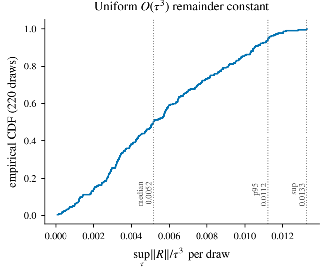
Fig. 9. Uniform remainder (arm ii): empirical CDF of the per-draw remainder constant \sup_\tau \|R\|/\tau^3 over 220 shape draws; the quoted 0.0133 is the supremum, not a typical value.
