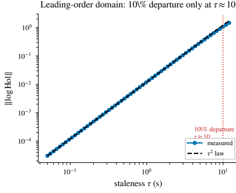
Fig. 11. Outside the leading-order domain: the measured amplitude departs from the \tau^2 law by 10% only at \tau \approx 10 — an order of magnitude beyond the operating grid ( \tau \leq 1.6 ), where the relative departure stays below 3.4 \times 10^{-3} . The theorem is a small- \tau statement and this is its measured boundary.
