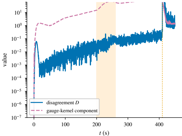
Maneuver excites D ; beacon kills the gauge, not D
